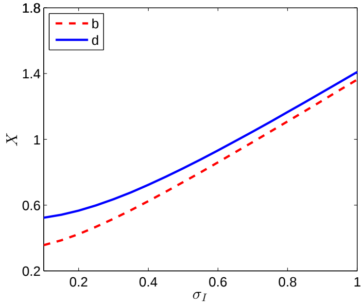
Figure 9: The effect of \sigma_I on trading volume X
