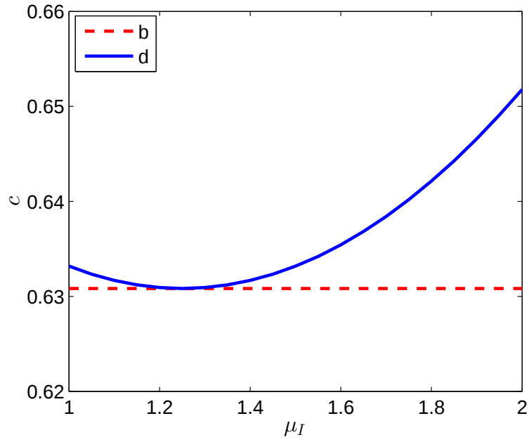
Figure 2: The effect of \mu_I on fee c
