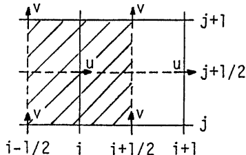
Fig. 4 Difference Scheme for x -wise Momentum Equation.
