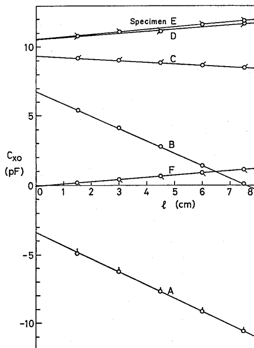
Fig. 11. Dependence of limiting capacitance C_{\infty 0} at low frequencies on the length l of the terminal leads for Specimens A, B, C, D, E and F.
