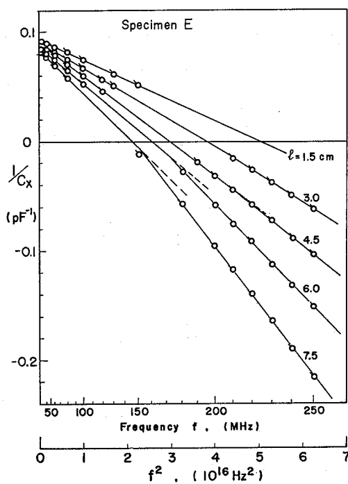
Fig. 9. Plots of the reciprocal of C_x against squared frequency f^2 for Specimen E, composed only of a capacitor, with varied length l of the terminal leads.
