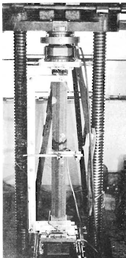
Fig. 6. Deformation measurement.
