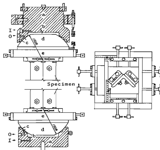
Fig. 4. End supports.
