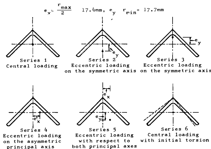
Fig. 3 (a). Eccentricities.
