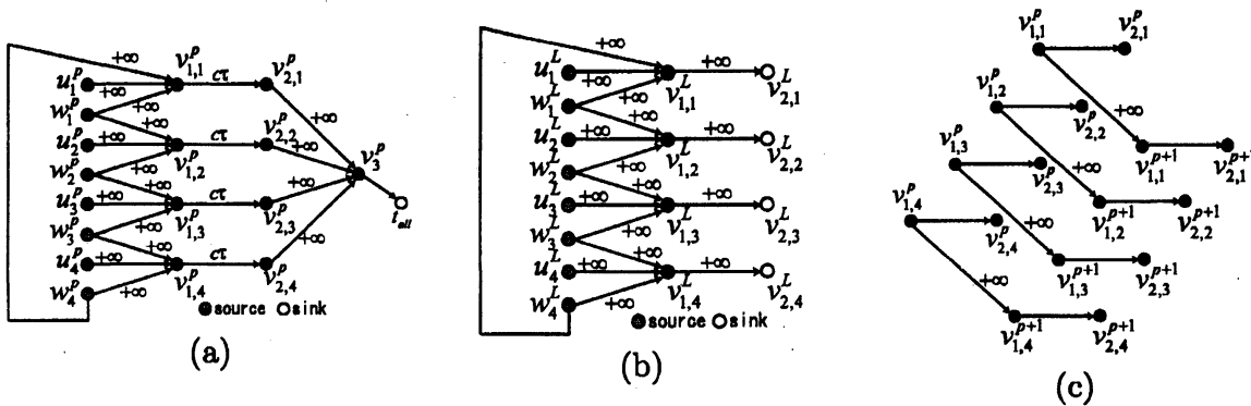
Figure 5: (a) p -th component C^p (b) L -th component C^m (c) p -th bridges
