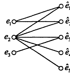
Figure 7: Bipartite graph of v in Fig 6
