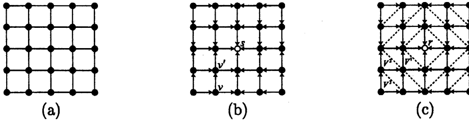
Figure 1: (a)Grid network (b)Direction of arcs (c)Layers of grid network
