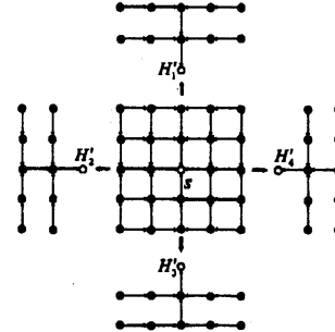
Figure 3: H'_1, H'_2, H'_3, H'_4
