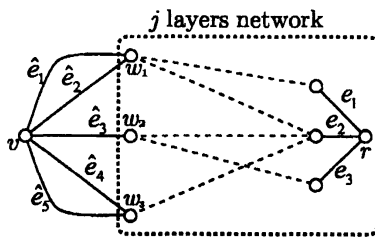
Figure 6: j + 1 -th layer
