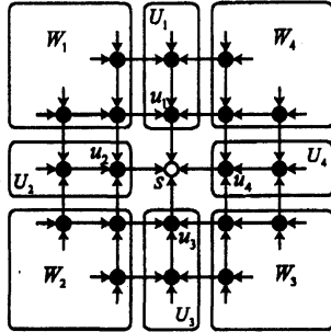
Figure 2: Decomposition of \mathcal{N}
