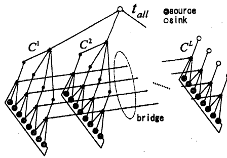
Figure 4: Illustration of the entire network constructed in Subsection 2.1
