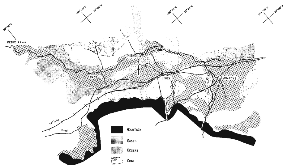
Fig. 1. Land feature map of HEIFE area and the location of stations. The (↑) arrow shows the test stations.
