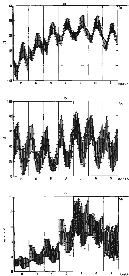
Fig. 5. Series of monthly mean diurnal courses (00–23 LT) and standard deviations (bars) of (a) air temperature ( T_a ), (b) relative humidity ( R_h ) and (c) specific humidity ( Sh ) from March to September, 1989.
