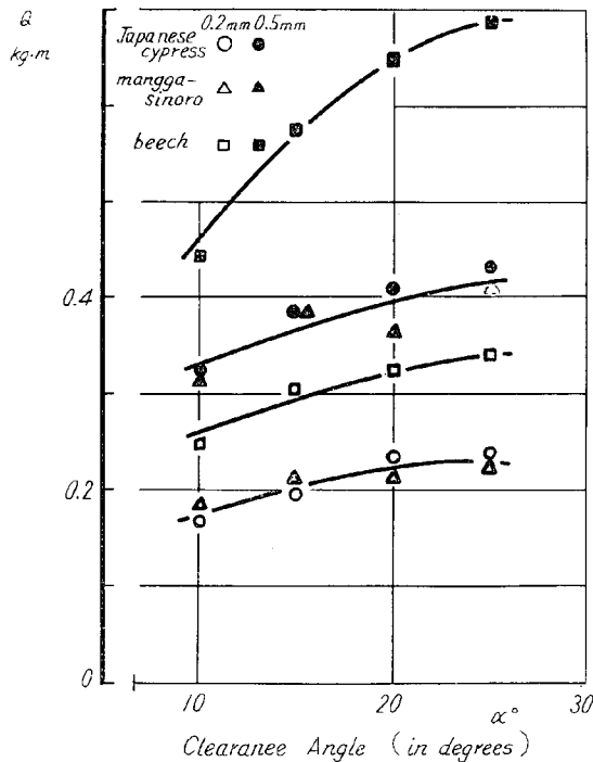
Fig. 22. Relation of Clearance Angle to Cutting Energy. (A x C x G)
