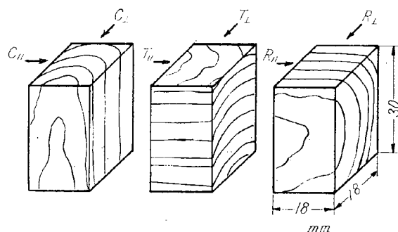
Fig. 4. Cutting Direction and Size of Test Block.
