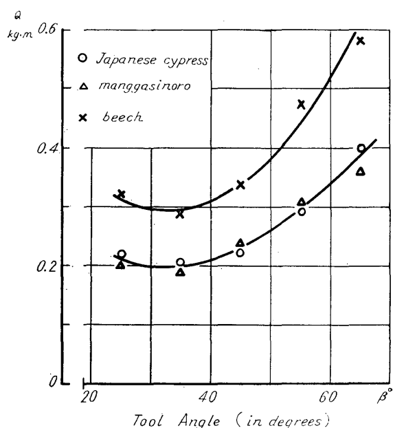
Fig. 11. Relation of Tool Angle to Cutting Energy. (A x F)
