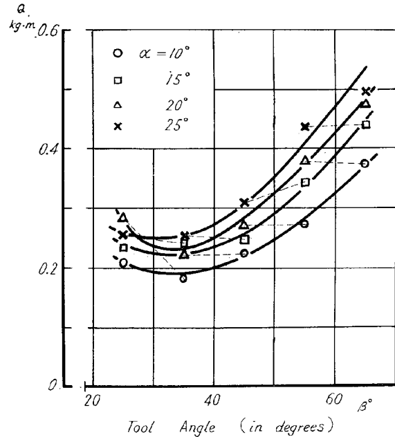
Fig. 23. Relation of Tool Angle to Cutting Energy. (F x G)
