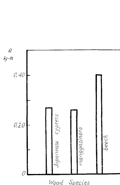
Fig. 5. Effect of Wood Species on Cutting Energy. (A)
