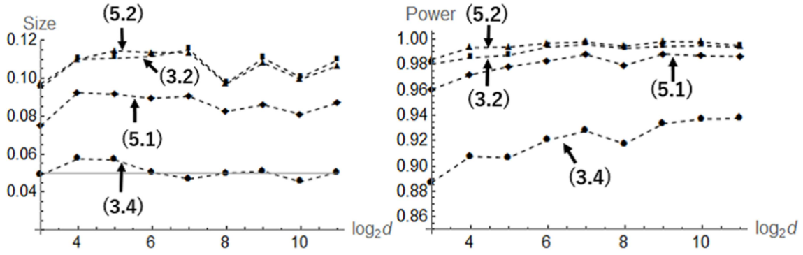
(I) d = 2^k ( k = 3, \dots, 11 ) and n_i = 10 .
