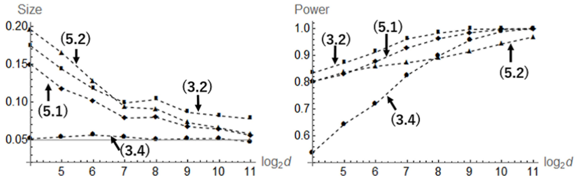
(II) d = 2^k ( k = 4, \dots, 11 ) and n_i = \lceil d^{1/2} \rceil , where \lceil x \rceil denotes the smallest integer \geq x .
