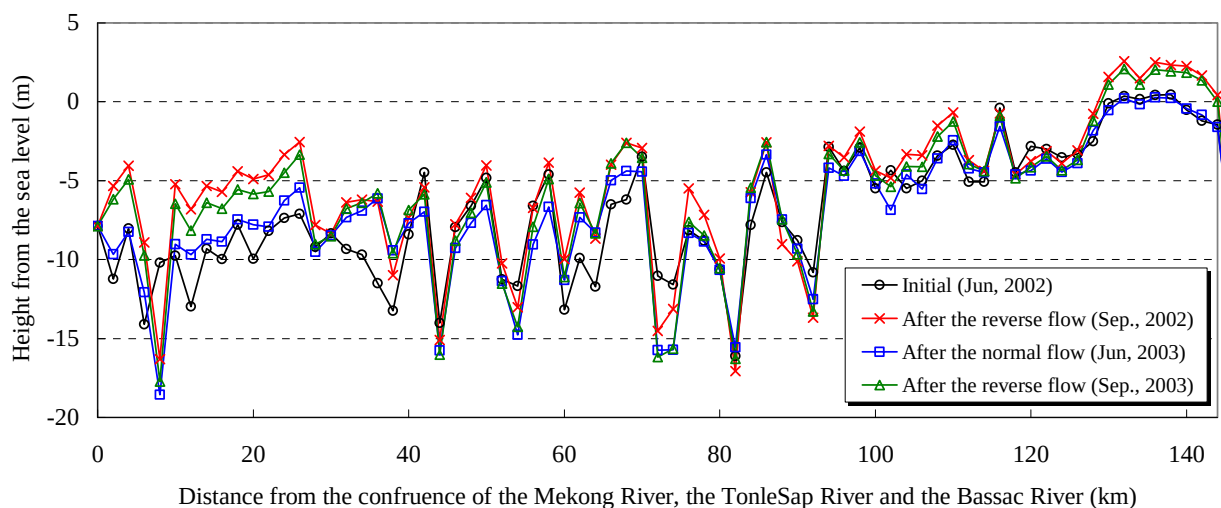
Fig. 13 Longitudinal distribution of deepest bed elevation in each cross-section
