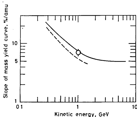
Fig. 5. Slope of the mass yield curve for spallation as a function of incident particle kinetic energy. Open point represents the result of 0.87 GeV \pi^- + \text{Bi} . Solid curve for \text{Cu} + \text{proton or heavy ion} and dashed curve for \text{Cu} + \pi^- are taken from Ref. 7) The pion points are plotted at an energy corresponding to the sum of their kinetic energy and the pion rest mass energy.
