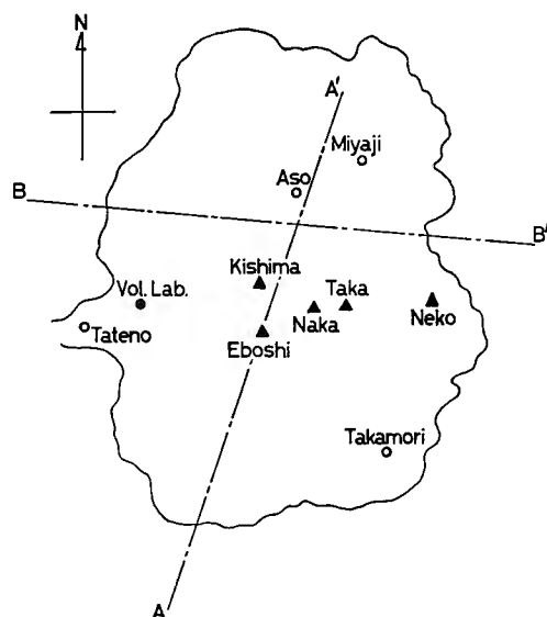
Fig. 6. Topographic map of the Volcano Aso. AA' and BB' show the dip directions of the southern and the northern block, respectively.
