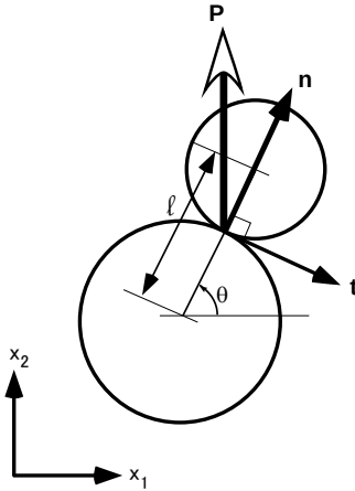
Fig. 1 Contact normal \mathbf{n} , tangential direction \mathbf{t} , and contact force \mathbf{P}
