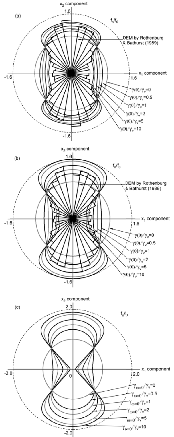
Fig. 6 Evolution of stress space fabric combined with isotropic fabric during biaxial shear; f_n / \bar{f}_0 (= 1 - r_n q / p^*) representing normal component of contact forces (DEM simulation by Rothenburg & Bathurst (Rothenburg and Bathurst, 1989) with modification); (a) r_n = 0.58 and \sin \phi_t = 0.43 , (b) r_n = 1.0 and \sin \phi_t = 0.43 , (c) r_n = 1.0 and \sin \phi_t = 0.64
