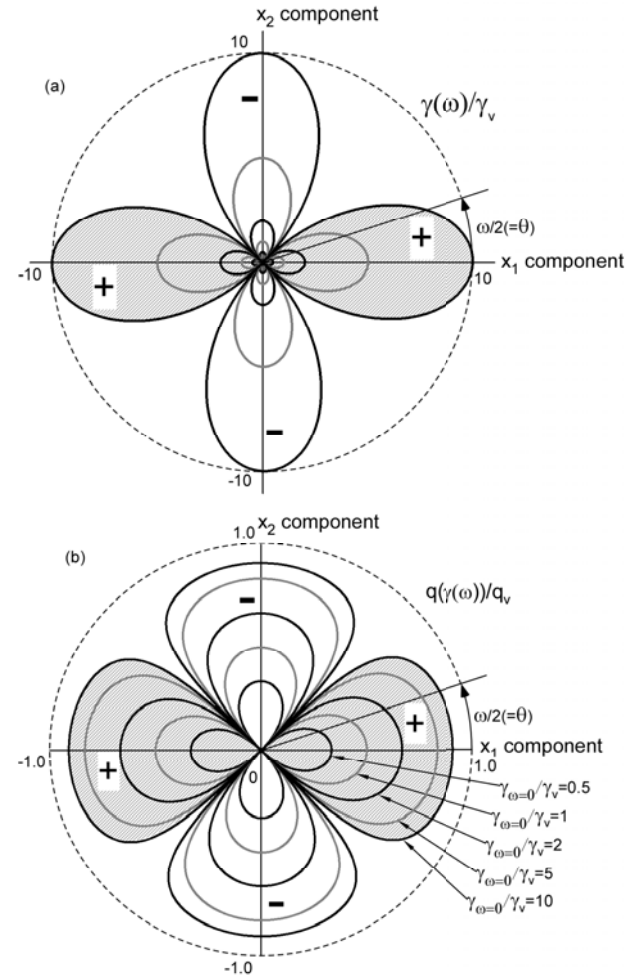
Fig. 4 Evolution of fabric during biaxial shear; (a) strain space fabric, (b) stress space fabric
