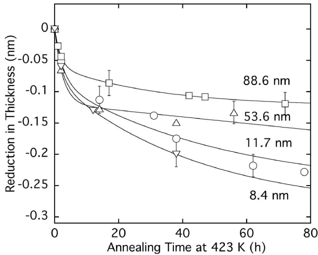
FIG. 3. Reduction in thickness as a function of annealing time at 423 K for various value of initial thickness d_0=88.6 ( \square ), 53.6 ( \triangle ), 11.7 ( \circ ), and 8.4 nm ( \nabla ). Solid curves are the results of fits with (d_\infty - d_0)[1 - A_f \exp(-t/\tau_f) - A_s \exp(-t/\tau_s)] .
