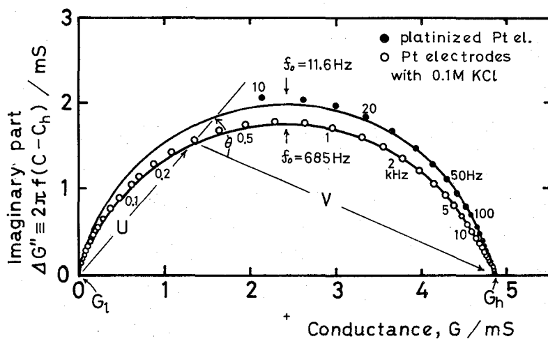
Fig.4 Complex plane plots of complex conductance [G, \Delta G^*] for the Pt electrode-KCl solution systems. The same data as shown in Fig.3. Filled circles \bullet are the observed data for a platinized Pt electrode cell filled up with a 0.1 M KCl solution, hollow circles \circ being for a Pt electrode (no Pt-black) system. The solid curves are calculated from Eqs. (12) and (13) using parameter values shown in Table I.
