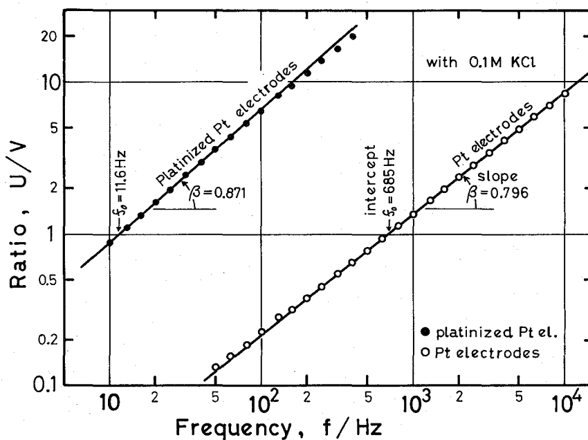
Fig.5 Plots of \log(U/V) against \log f for the data shown in Figs.3 and 4. Filled circles \bullet are the observed data for a platinized Pt electrode cell filled up with a 0.1 M KCl solution, hollow circles \circ being for a Pt electrode (no Pt-black) system.
