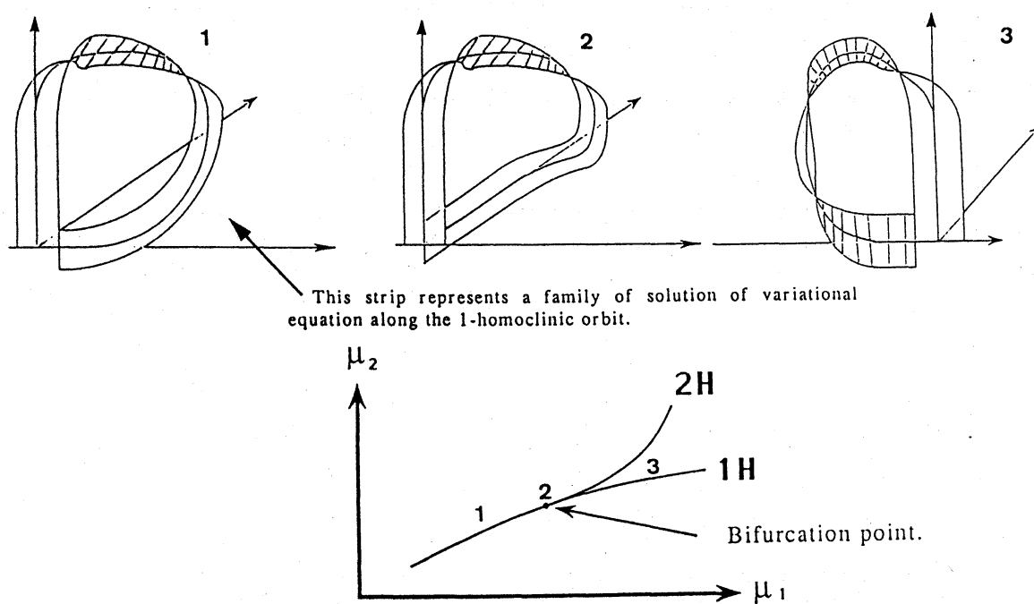
Fig 3 Non - principal homoclinic orbit
