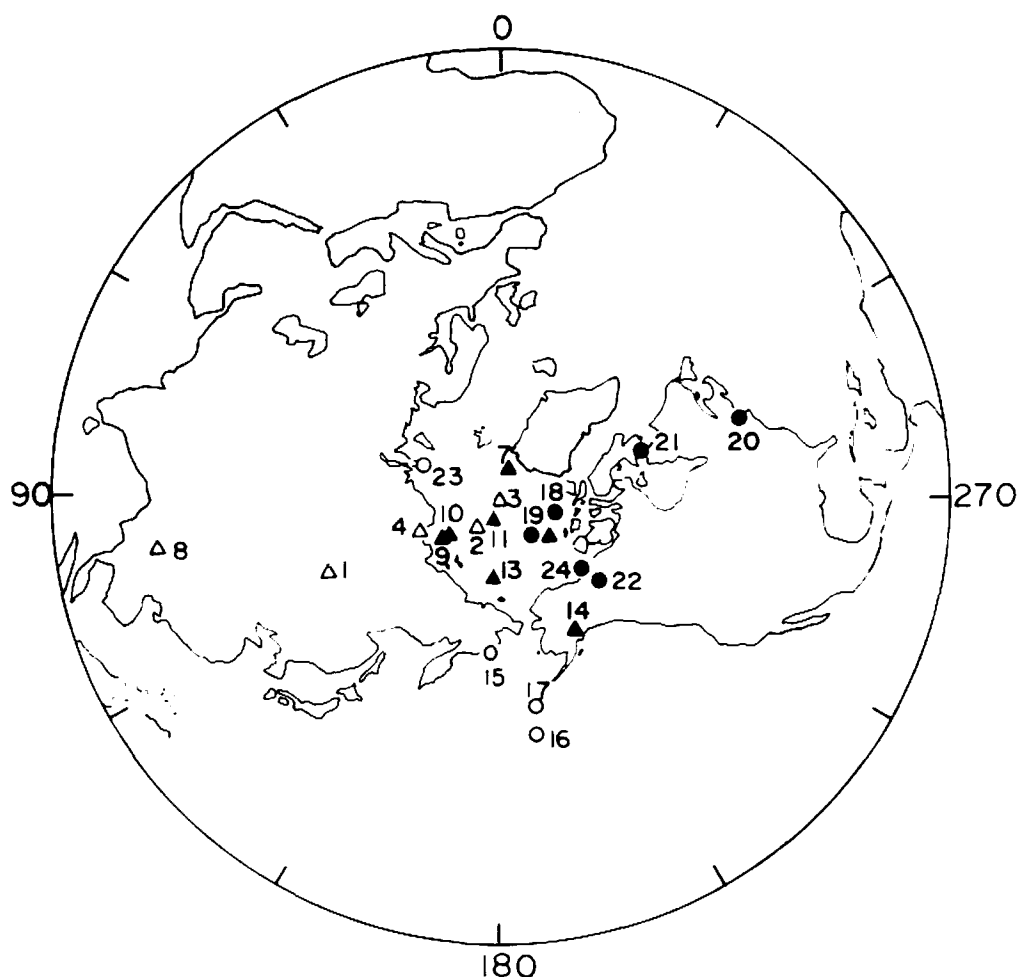
Fig. 7 VGPs plotted on polar equal area projection of Northern Hemisphere. Triangle and circle symbols are from the Nachola and Aka Aiteputh Formations, respectively. Numbers indicate Site Nos. in Table 1. Solid symbols correspond to north poles, and open symbols to south poles.
