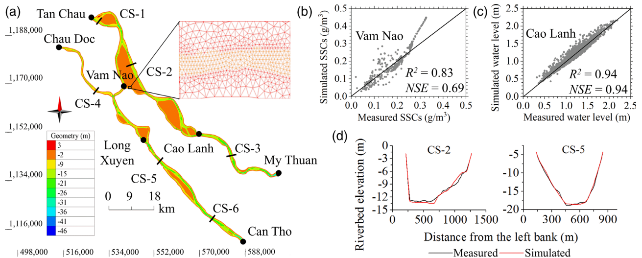
FIGURE 3 (a) Simulated domain, mesh, geometry and boundaries of the coupled Telemac-2D and Sisyphe model. (b)–(d) validation results: Relations between simulated and measured daily SSCs, daily water levels and riverbed elevations. These results indicate that the model was well validated. NSE = Nash-Sutcliffe coefficient
