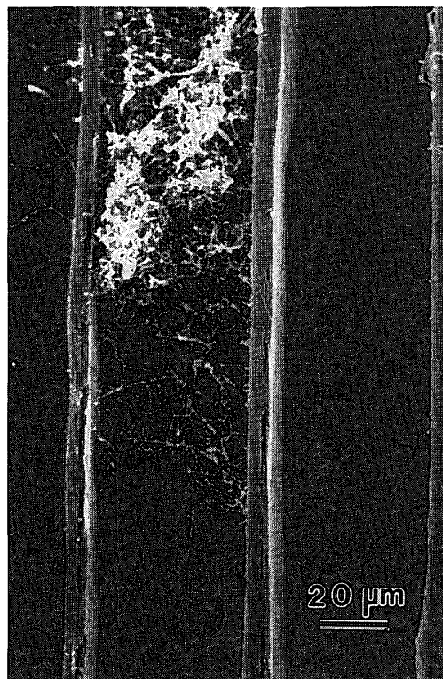
Fig. 1.9. Scanning electron micrograph of sugi tracheids at the surface portion of treated block after exposure to Tyromyces palustris . The cell lumina allowed to colonization with fungal hyphae, but the cell walls were not destructed and maintained the intact conditions.
