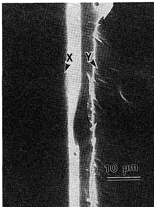
Fig 1.20. The lumen surface of tracheids of DMDHEU-treated wood. The left cell lumen (X) had no deposit of DMDHEU in spite of the full deposits in adjacent cell lumen (Y).
