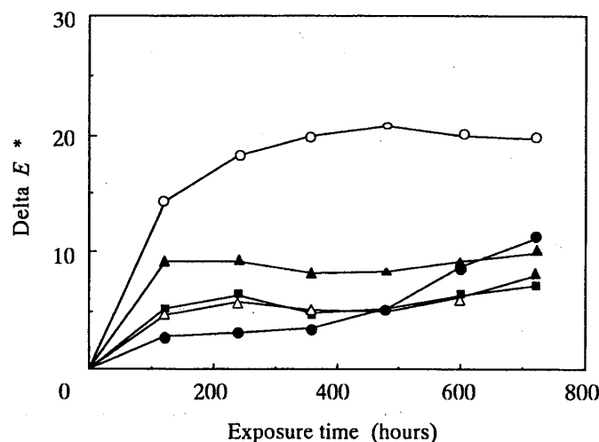
Fig 1.27. Color difference of finished LVLs treated with cross-linking reagents after artificial exposure for 720 hrs. Note and Legend: See Fig. 1.25.
