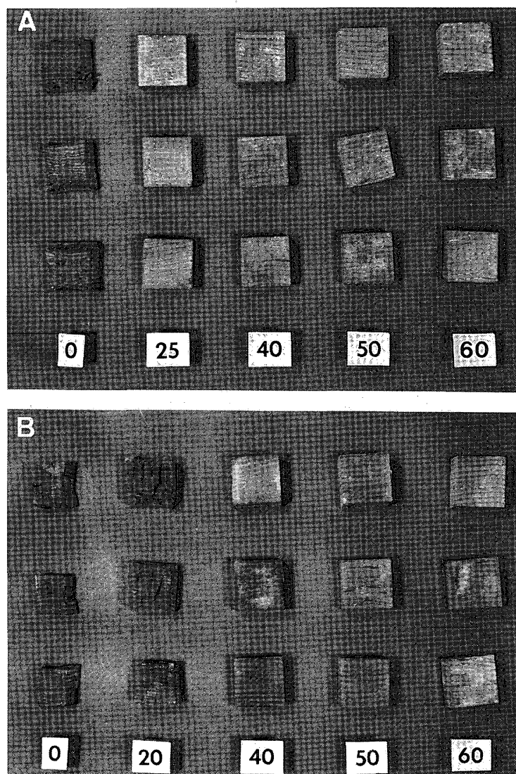
Fig. 1.11. The vapor-phase formaldehyde-treated western hemlock after decay test of Coriolus versicolor (a) and Tyromyces palustris (b) for 12 weeks.
