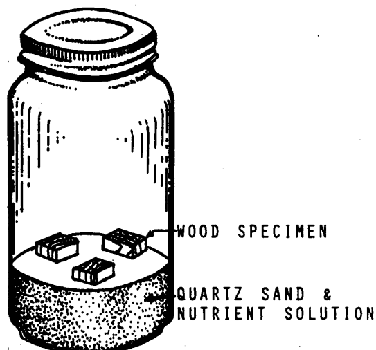
Fig. 1.2. An assembled soil block test according to JWPA No.3-1992.
