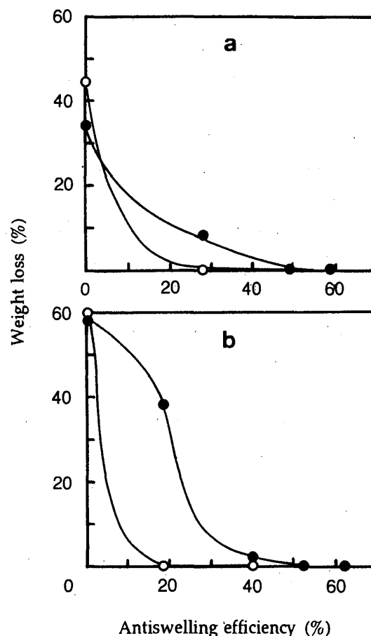
Fig. 1.10. The relationship between antismelling efficiency and weight loss of formaldehyde-treated sugi (a) and western hemlock (b) after exposure to fungi for 12 weeks. Legend: ●: Tyromyces palustris , ○: Coriolus versicolor .
