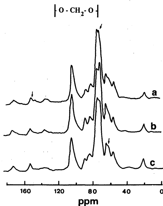
Fig. 1.17. 13 C NMR spectra of formaldehyde-treated sugi. Legend: a: 50% of ASE, b: 20% of ASE, and c: Control.
