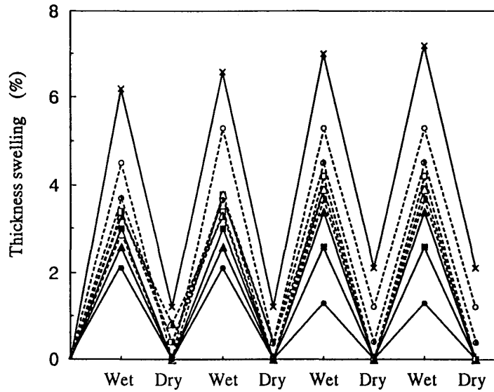
Fig. 2.6. Thickness swelling of untreated and treated LVLs after 4-cycle dry and wet aging test.
