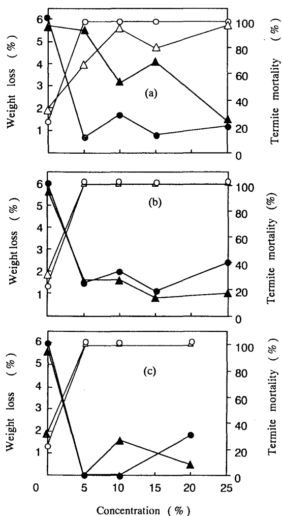
Fig 1.24. Average weight loss (WL) of glutaraldehyde-(a), DMDHEU-(b), and glyoxal-(c) treated wood and mortality (TM) of workers after exposure to termite of Reticulitermes speratus for 3 weeks.
