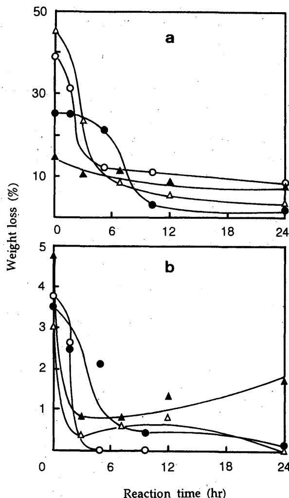
Fig. 1.12. Weight loss of formaldehyde-treated wood in vapor phase after exposure to Coptotermes formosanus for 9 weeks (a), Reticulitermes speratus for 3 weeks (b). Legend: See Fig. 1.4.
