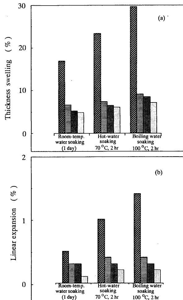
Fig. 2.8. The thickness swelling (a) and linear expansion (b) of waferboards treated with vapor phase formalization at different water soaking conditions. Legend: Control, 2.9% WG, 3.0% WG, and 3.1% WG.
