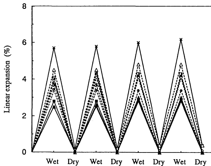
Fig. 2.7. Linear expansion of untreated and treated LVLs after 4-cycle dry and wet aging test.
