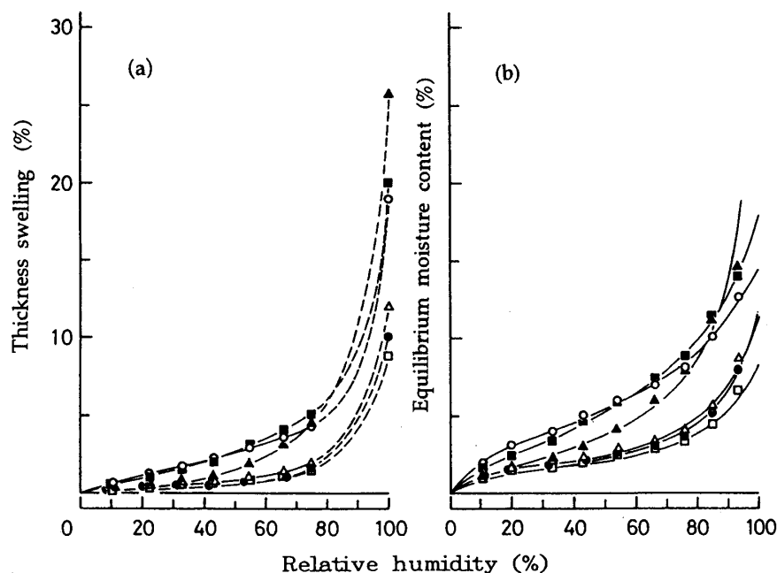
Fig. 2.13. Dependence of thickness swelling (a) and equilibrium moisture content (b) of formaldehyde-treated S-MDF on the relative humidity.
