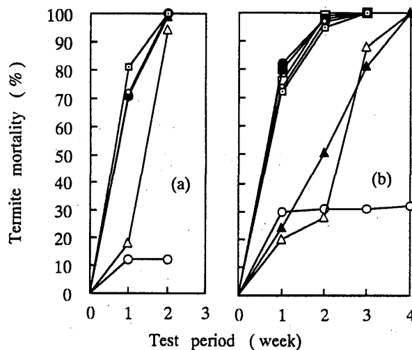
Fig. 1.16. Mortality of worker termite of Reticulitermes speratus fed on formaldehyde-treated sugi (a) and buna (b). Legend: See Fig 1.15.
