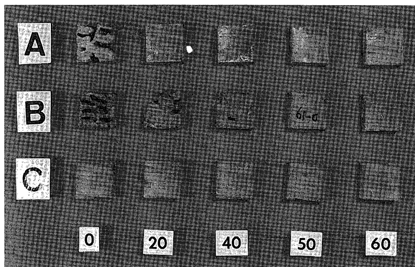
Fig. 1.13. The formaldehyde-treated sugi in vapor phase after attack to subterranean termite. Legend: A: Choice tests with Coptotermes formosanus , B: Forced-feeding tests with Coptotermes formosanus , and C: forced-feeding test with Reticulitermes speratus . Note: The number at the bottom show the values of ASE.
