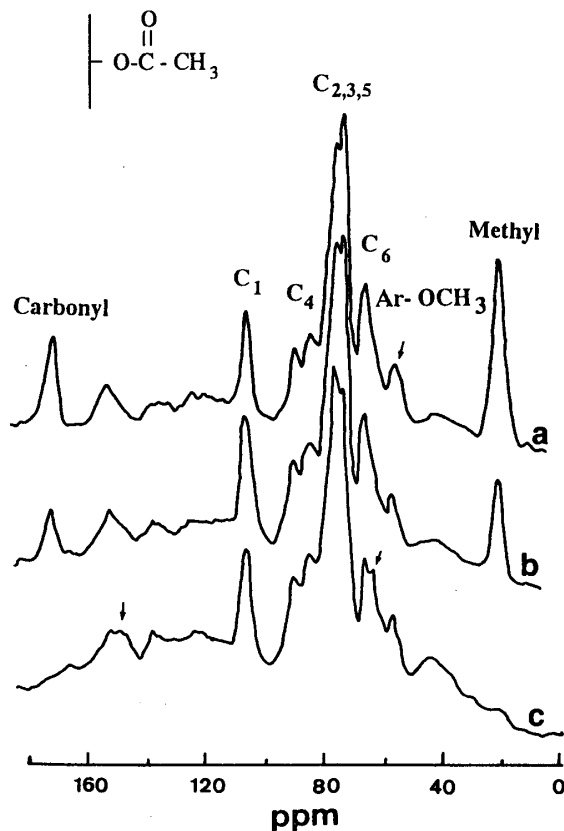
Fig. 1.18. ^{13}\text{C} NMR spectra of acetylated sugi (cited from Takahashi et al. 14) Legend: a: 20% of WG, b: 10% of WG, and c: Control.
