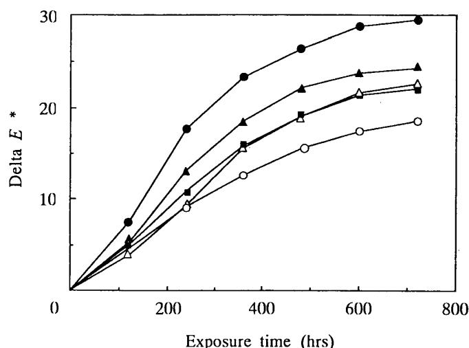
Fig 1.28. Color difference of finished LVLs treated with cross-linking reagents after artificial exposure for 720 hrs. Note and Legends: See Fig. 3.1.
