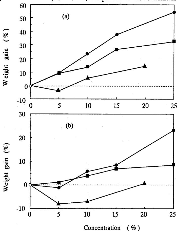
Fig 1.19. Relationship between concentration of solution and weight gain (WG) of treated sugi (a) and buna (b).
