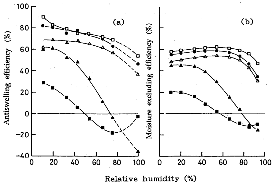
Fig. 2.14. Dependence of antiswelling efficiency (a) and moisture excluding efficiency (b) of formaldehyde-treated S-MDF on the relative humidity. Legend: See Fig. 2.13.
