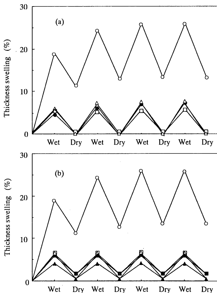
Fig. 2.10. The thickness of the treated and untreated waferboards during accelerated aging test of 4-cycle soak-dry.
