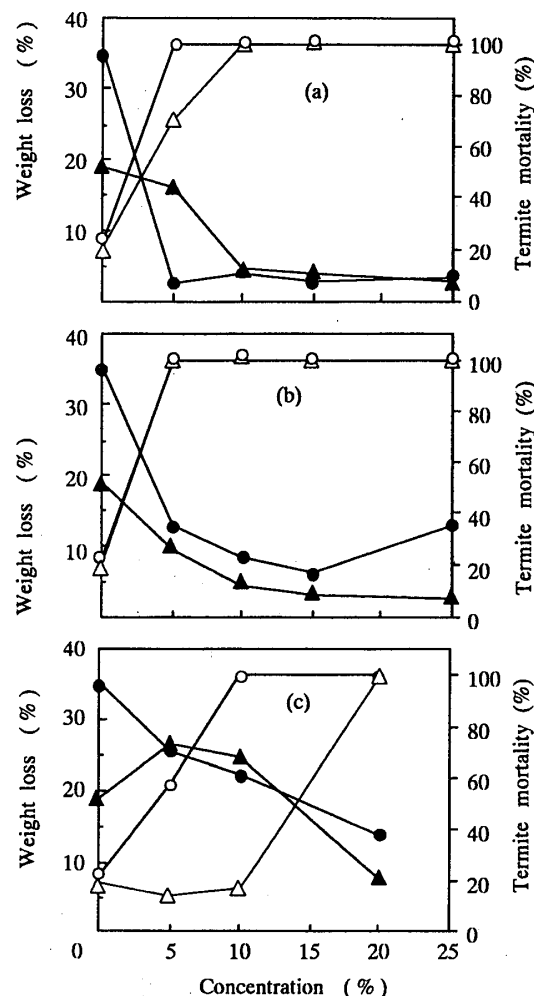
Fig 1.23. Average weight loss (WL) of glutaraldehyde-(a), DMDHEU-(b), and glyoxal-(c) treated wood and mortality (TM) of workers after exposure to termite of Coptotermes formosanus for 9 weeks.
