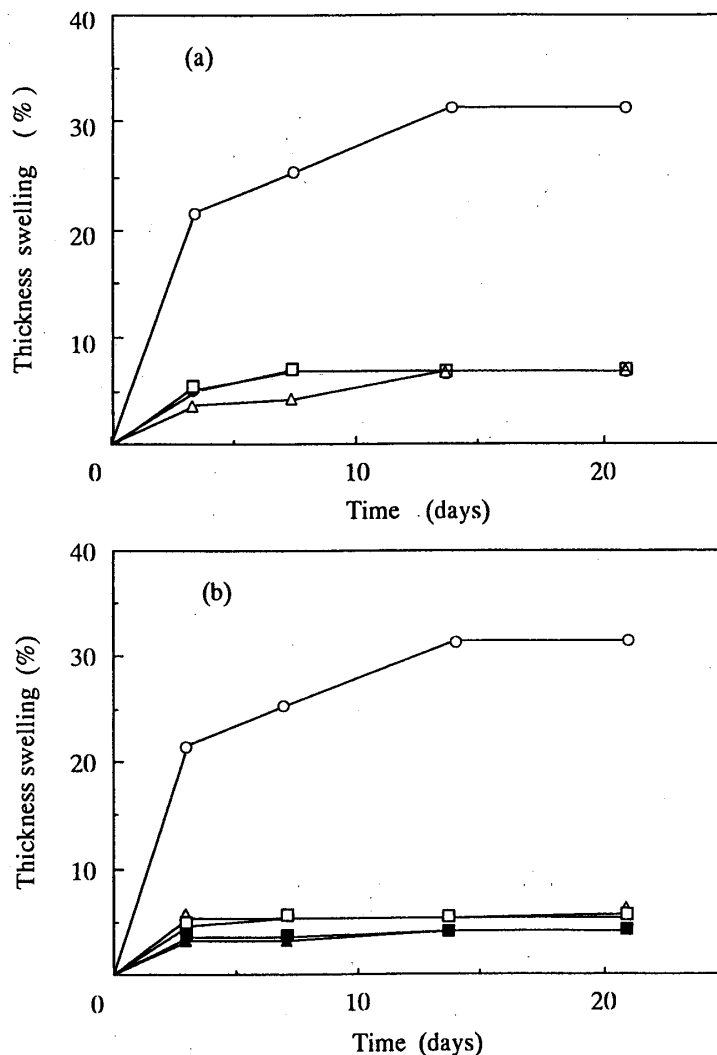
Fig. 2.11. The thickness of the treated and untreated waferboards during water soaking at room temperature. Legend: See Fig. 2.10.
