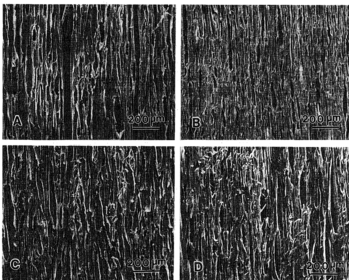
Fig 1.29. SEM observations of the unfinished surface of untreated (A), tetraoxane (B), DMDHEU (C) and glutaraldehyde (D) treated LVLs after exposure to artificial weathering for 720 hrs.
