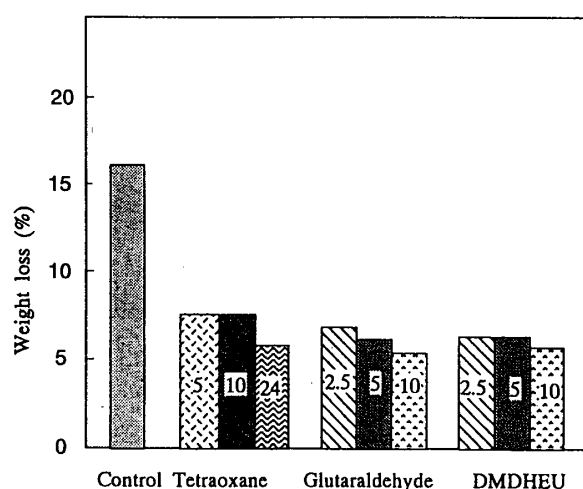
Fig. 2.2. The weight loss of cross-linking agents-treated veneer of LVLs after exposed to termite attack of Coptotermes formosanus for 9 weeks.
