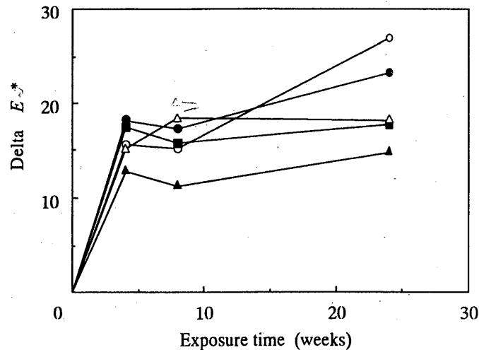
Fig 1.26. Color difference of finished LVLs treated with cross-linking reagents after outdoor exposure for 24 weeks. Note and Legend: See Fig. 1.25.
