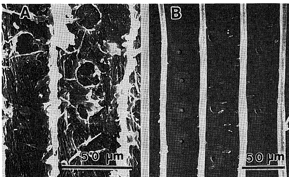
Fig. 1.7. Scanning electron micrographs of untreated (A) and formaldehyde-treated sugi tracheids (B) after 9-month exposure in unsterilized moist soil.
