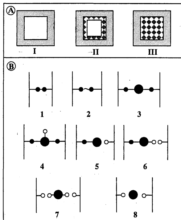
Model of chemical modification of wood. A, cellular level; (I) modification of cell wall only, (II) deposition on lumen surface, (III) filling up of lumen. B, modification of lignocellulosic material at molecular level. Empty circles, hydroxyl group available for hydrogen bonding; small filled circles, substitution of hydroxyl group; large filled circles, bulking agent (cited from Norimoto et al. 1) , with permission).
