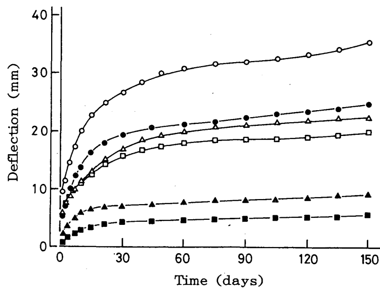
Fig. 2.17. Deflection-time curves of untreated and formaldehyde-treated MDF in bending creep test under progressive attack by Tyromyces palustris .
