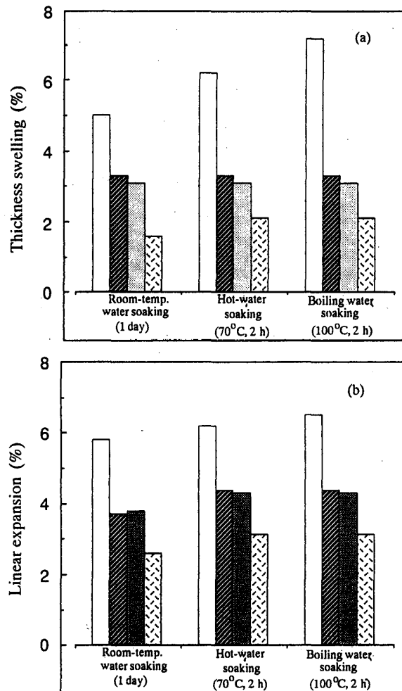
Fig. 2.5. Thickness swelling (a) and linear expansion (b) of DMDHEU-treated LVLs after water immersion. Legend: See Fig. 2.3.
