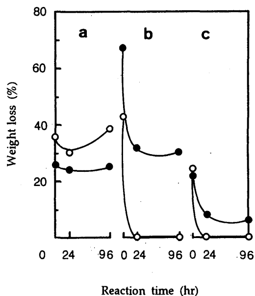
Fig. 1.8. Weight loss of formaldehyde-treated wood in liquid phase after decay for 12 weeks by Tyromyces palustris (a), Coriolus versicolor (b), and soil burial test (c) for 9 months. Legend: See Fig. 1.4.
