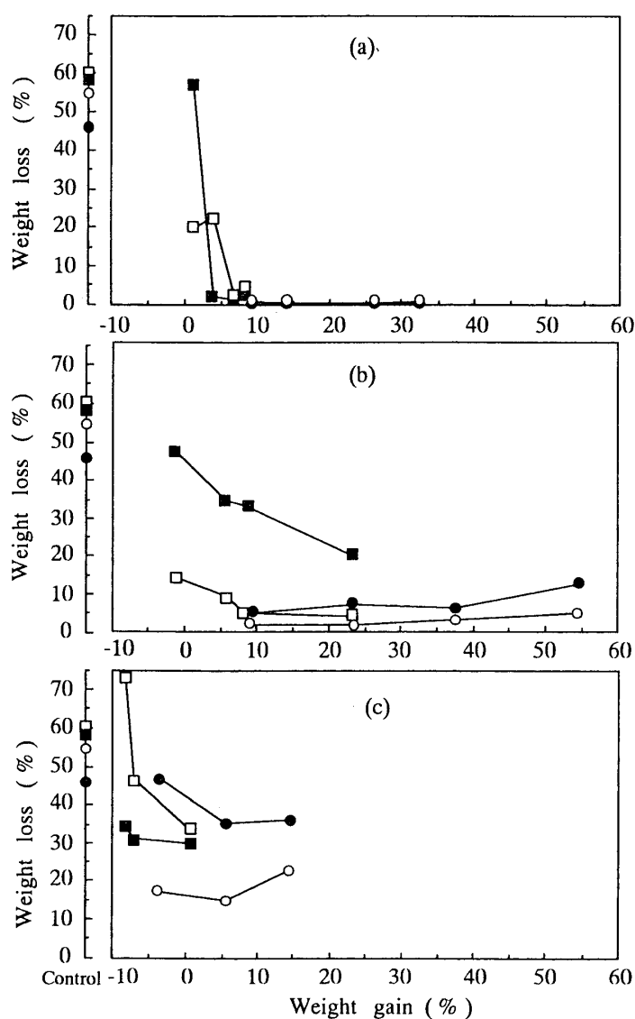
Fig 1.22. Average weight loss of glutaraldehyde- (a), DMDHUE-(b) and glyoxal- (c) treated wood after exposure to decay fungi for 12 weeks.
