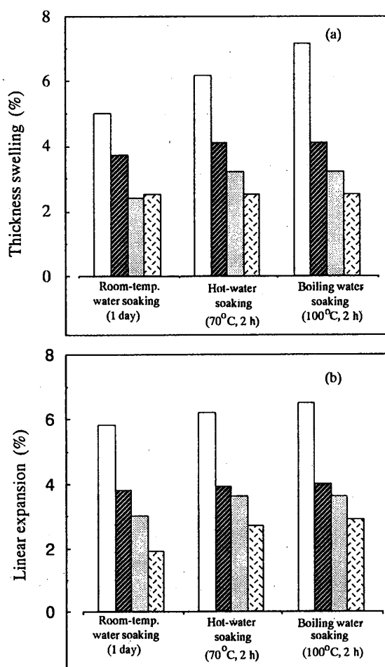
Fig. 2.3. Thickness swelling (a) and linear expansion (b) of formaldehyde-treated LVLs after water immersion.
