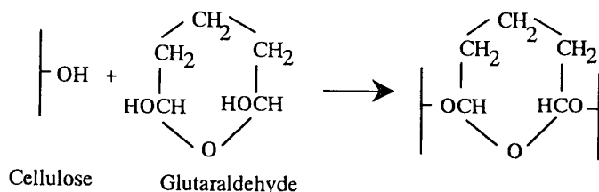
Scheme 1.2. Proposed cross-linking linkages between cellulose and glutaraldehyde (cited from Frick et al. 25)
