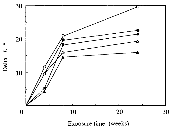
Fig 1.25. Color difference of unfinished LCVLs treated with cross-linking agents after outdoor exposure for 24 weeks.
