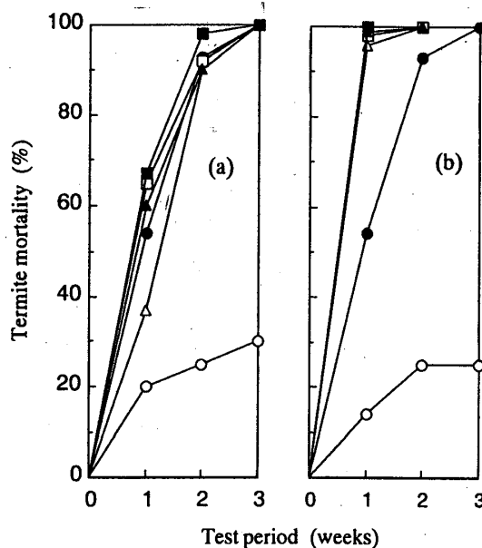
Fig. 2.19. Mortality of worker termite of Reticulitermes speratus fed on softwood (a) and hardwood MDFs (b). Legend: See Fig. 2.18.
