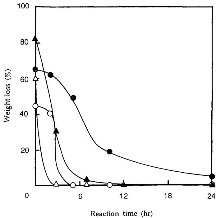
Fig. 1.5. Weight loss of formaldehyde-treated wood in vapor phase after exposure to white-rot fungus Coriolus versicolor for 12 weeks. Legend: See Fig. 1.4.
