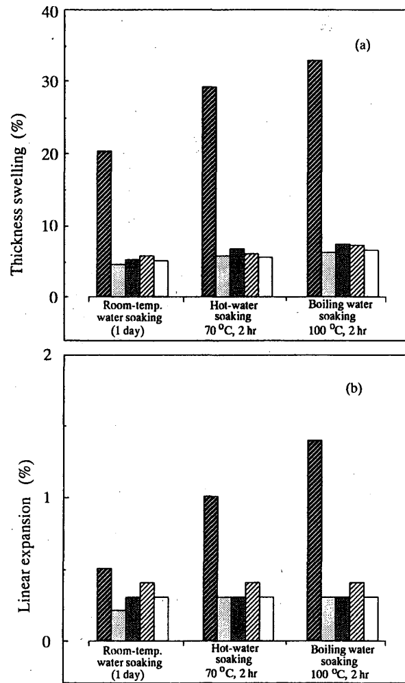
Fig. 2.9. The thickness swelling (a) and linear expansion (b) of waferboards treated with pad-dry-cure treatments at different water soaking conditions.
