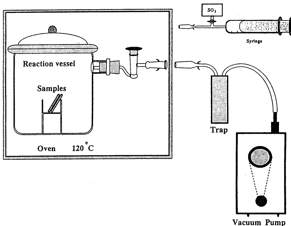
Fig. 1.1. Equipment for the vapor phase formalization.
