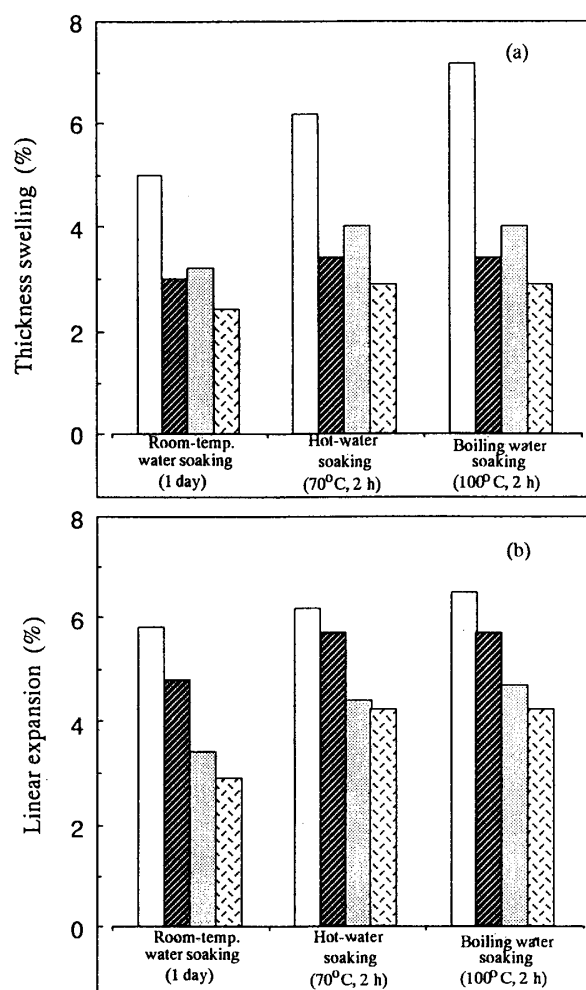
Fig. 2.4. Thickness swelling (a) and linear expansion (b) of glutaraldehyde-treated LVLs after water immersion.
