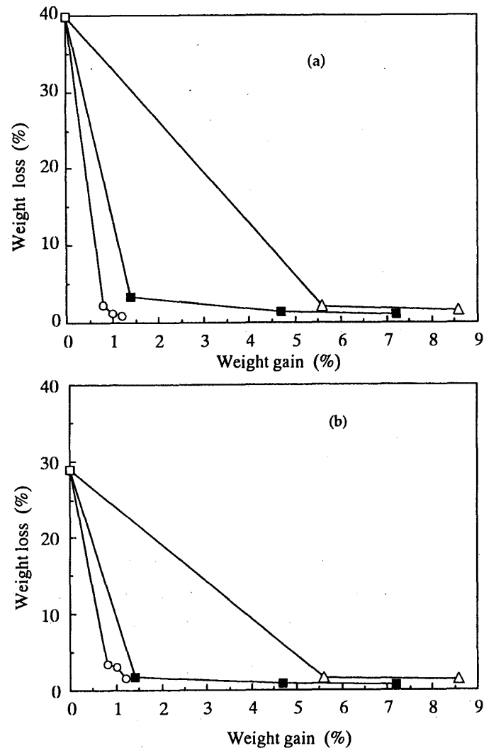
Fig. 2.1. The WL of LVLs treated with cross-linking reagent after 12 weeks exposure to Tyromyces palustris (a) and Coriolus versicolor (b). Legend: ○: Formaldehyde, ■: glutaraldehyde, △: DMDHEU, □: Untreated.
