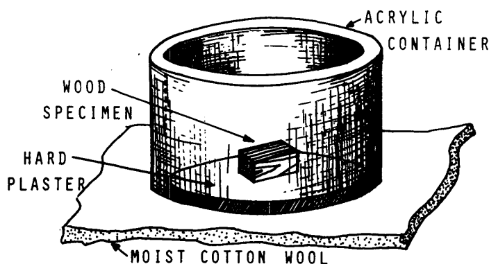
Fig. 1.3. An assembled forced-feeding test according to JWPA Standard No. 12-1992.
