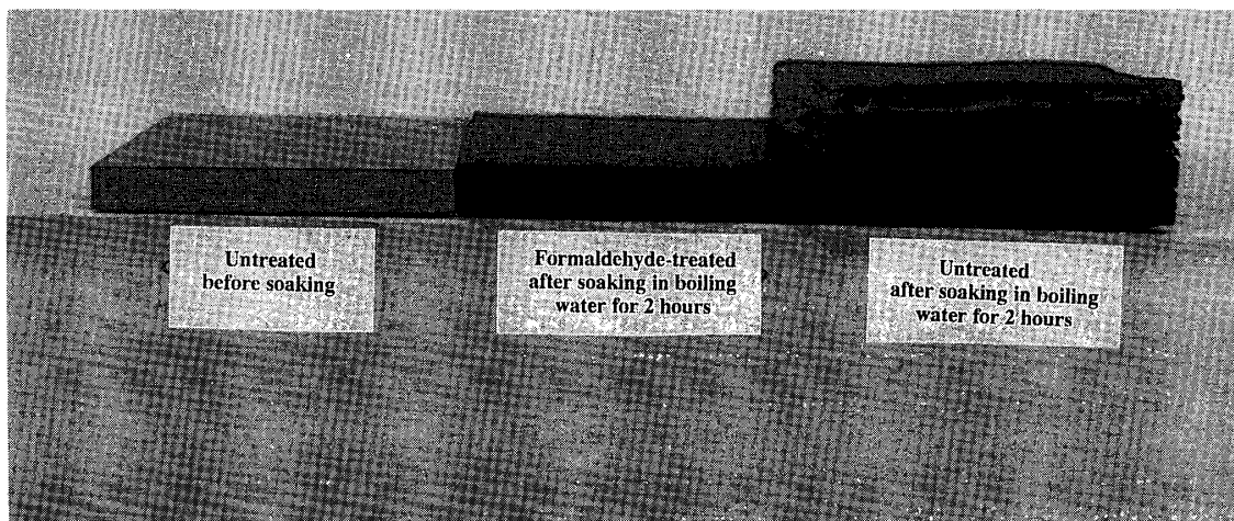
Fig. 2.15. The swelling of the untreated and formaldehyde-treated S-MDFs after soaking at boiling water for 2 hr (Photo: by K. Minato and his courtesy).
