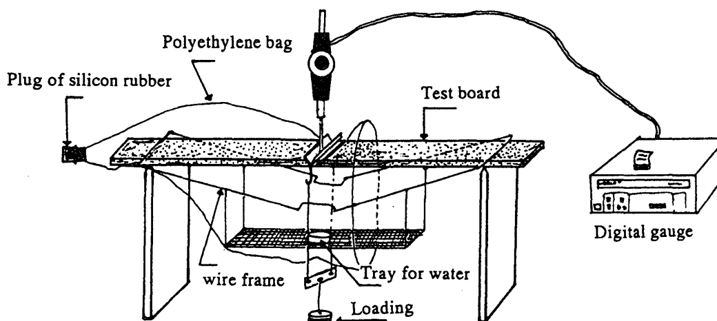
Fig. 2.12. Equipment for bending creep test under fungal attack of Tyromyces palustris .
