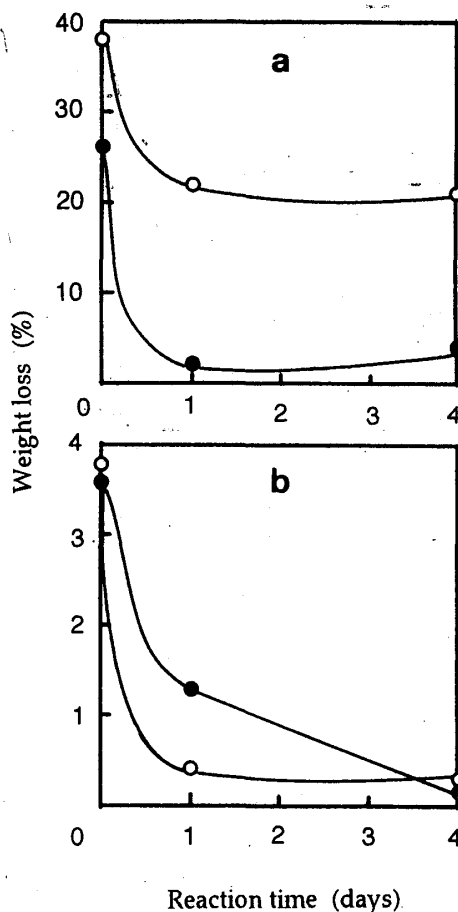
Fig. 1.14. Weight loss of formaldehyde-treated wood in liquid phase after exposure to Coptotermes formosanus for 9 weeks (a), and Reticulitermes speratus for 3 weeks (b). Legend: See Fig. 1.4.
