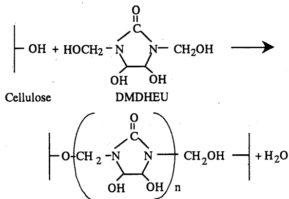
Scheme 1.4. Proposed linkage between DMDHEU and cellulose (cited from Frick et al. 34) )
