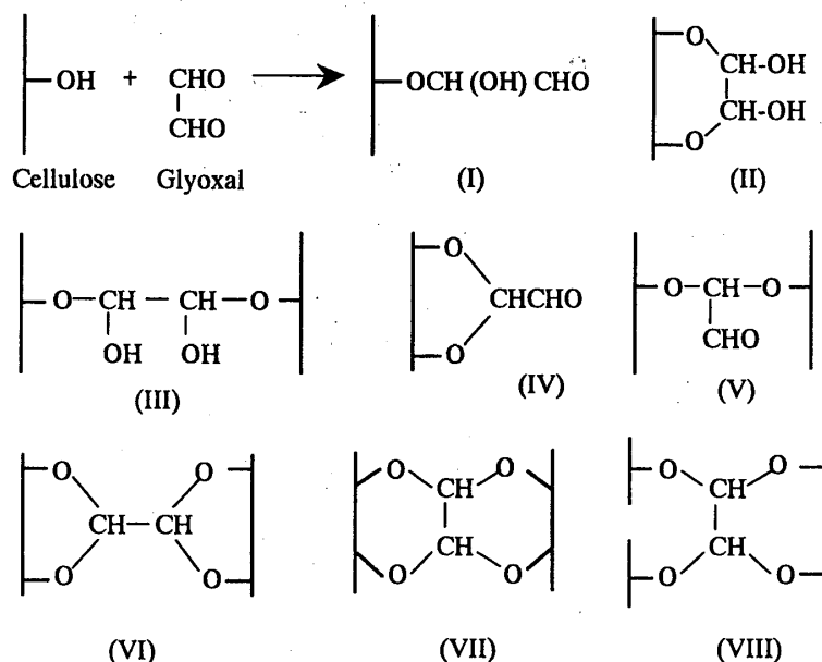
Scheme 1.3. Proposed cross-linking linkages between cellulose and glyoxal (cited from Head et al. 23) )
