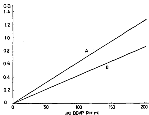
Fig. 1. Spectrophotometric determination of DDVP. A: in the absence of the digestive juice, measured at 218\text{m}\mu , B: in the presence of the digestive juice, measured at 230\text{m}\mu .
