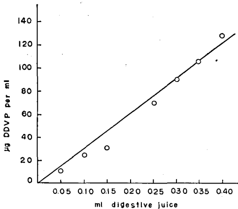
Fig. 4. Relationship between the amount of DDVP formed from trichlorofon and the amount of the digestive juice added during 5 minutes reaction at pH 7.0. Value of DDVP formation with each amount of the digestive juice was subtracted by that of the zero-time reaction.
