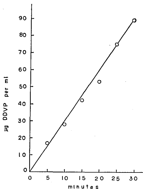
Fig. 3. Time course of DDVP formation from trichlorofon in the digestive juice at pH 7.0. Value of DDVP formation at each reaction time was subtracted by that obtained at zero time.
