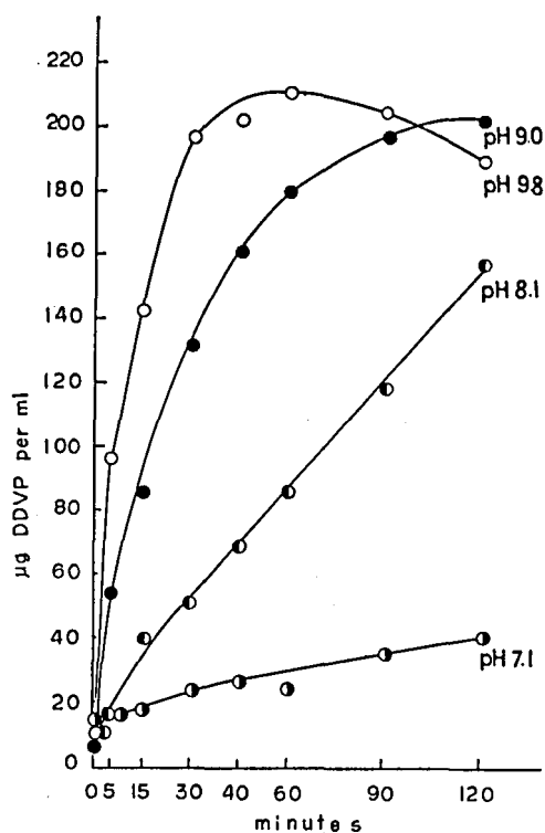
Fig. 2. The amount of DDVP converted non-enzymically from 2.57 mg of trichlorofon in various pH solutions.
