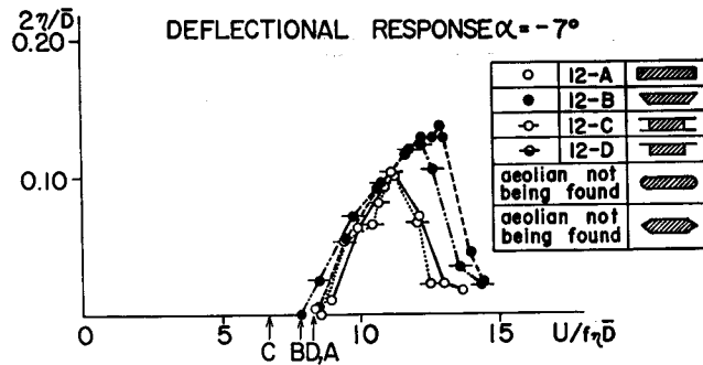
Fig. 8 Response Characteristics
