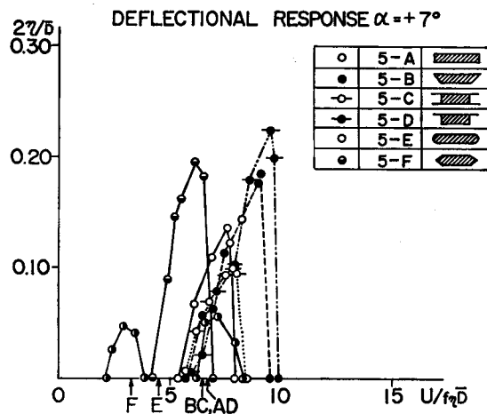
Fig. 4 Response Characteristics
