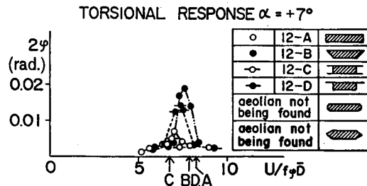
Fig. 9 Response Characteristics
