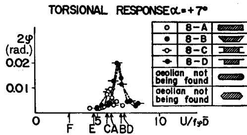
Fig. 7 Response Characteristics
