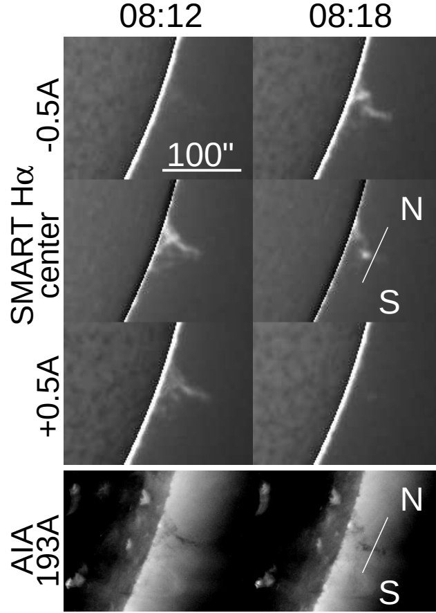
Fig. 4.— Temporal evolution of the oscillating prominence. From top to bottom : H\alpha -0.5 Å, center images, and +0.5 Å images taken by SMART, and EUV 193 Å images taken by SDO/AIA . The field of view of each panels is the region P shown in Figure 1. The times (UT) are indicated on the top.
