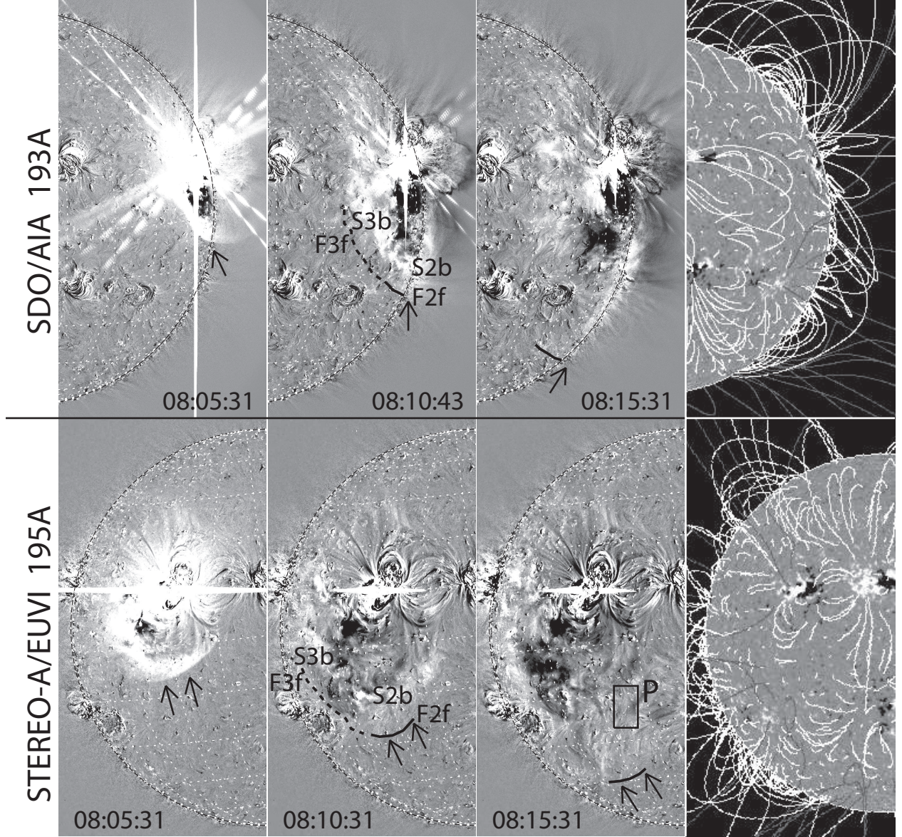
Fig. 2.— EUV waves observed with SDO /AIA 193 Å ( top ) and STEREO-A /SECCHI/EUVI 195 Å ( bottom ). The arrows follow the front of the EUV fast coronal wave. The region with mark P points the position of the limb prominence. The right panels show the potential magnetic field lines for the views from the earth ( top right ) and from the STEREO-A ( bottom right ).
