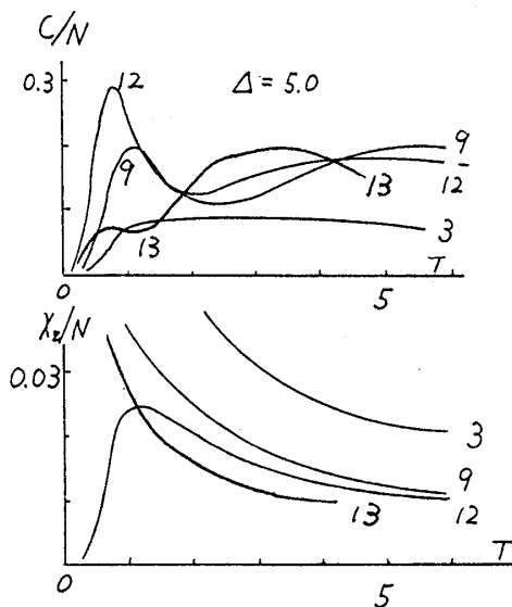
図9 Ising-like model
