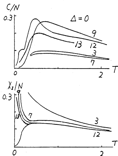
図8. XY model
