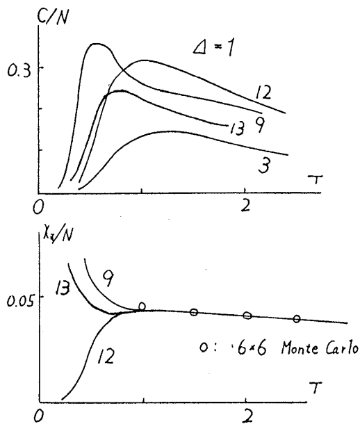
図7. Heisenberg model
