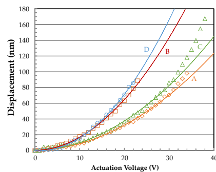
Figure 7. Measured displacement of all of the specimens A–D against applied actuation voltage on the electrostatic actuator. Specimens were fractured at the highest voltage of the plots. Fitting lines indicate quadratic function.
