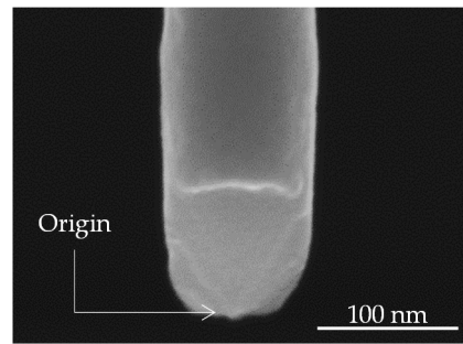
Figure 8. Fracture surface of Specimen A.
