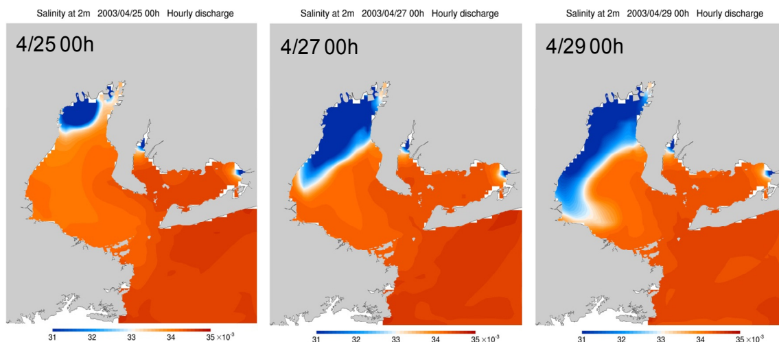
Fig.8 Distribution of sea surface salinity (25, 27 and 29/Apr/2003)
