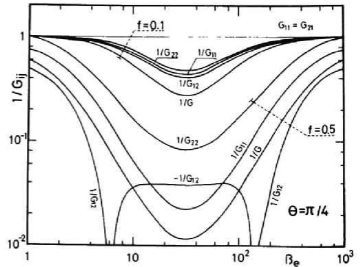
Fig.1.5. 1/G_{ij} vs. \beta_e for \theta = \pi/4 .
