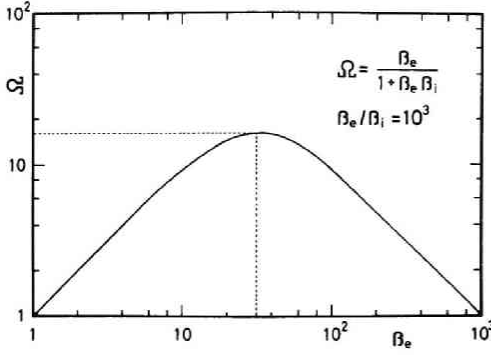
Fig.1.2. \Omega vs. \beta_e .
