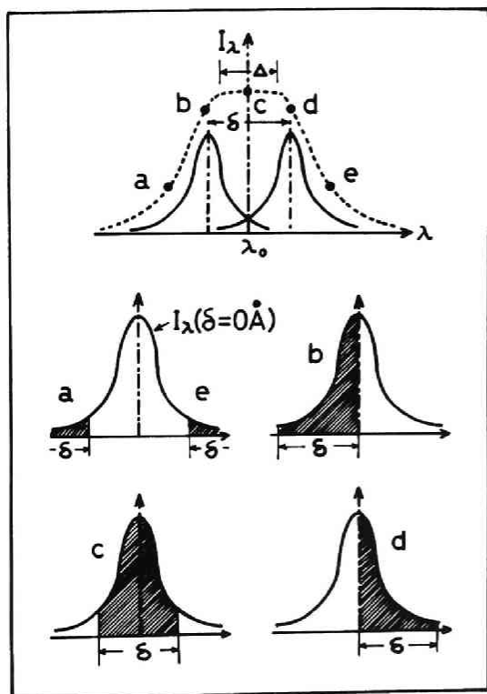
Fig.5.4. Distorted spectral shape(dotted curve) on the focal plane of the spectroscopy.
