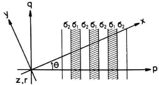
Fig.1.1. Coordinate system and nonuniformity. Plasma flows in the positive x direction and magnetic field is applied in the positive z direction.
