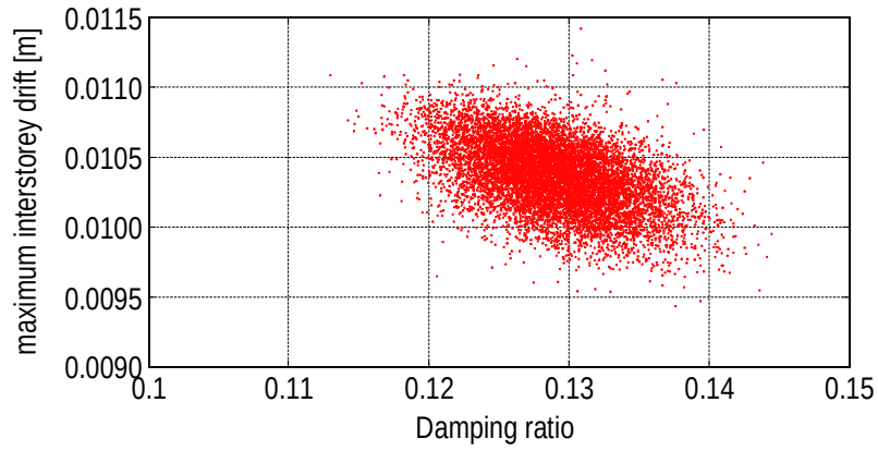
Fig.12 Distribution of maximum interstorey drift of damped structures given by randomly generated structural parameters (El Centro NS (1940))
