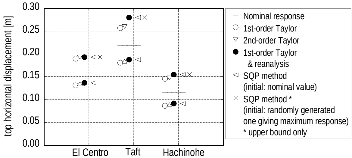
Fig.7 Comparison of evaluated bounds of top horizontal displacement under uncertain structural parameters derived by Taylor series approximations with those derived by SQP method
