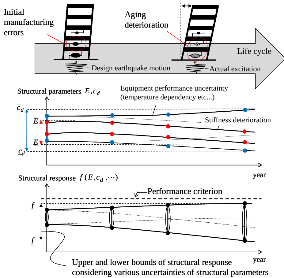
Fig.1 Concept of sustainable design considering varied structural performance caused by various uncertainties of structural parameters
