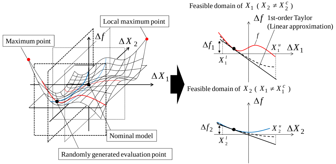
Fig.4 Concept of advanced interval analysis method using Taylor series approximation and random search technique for initial evaluation point
