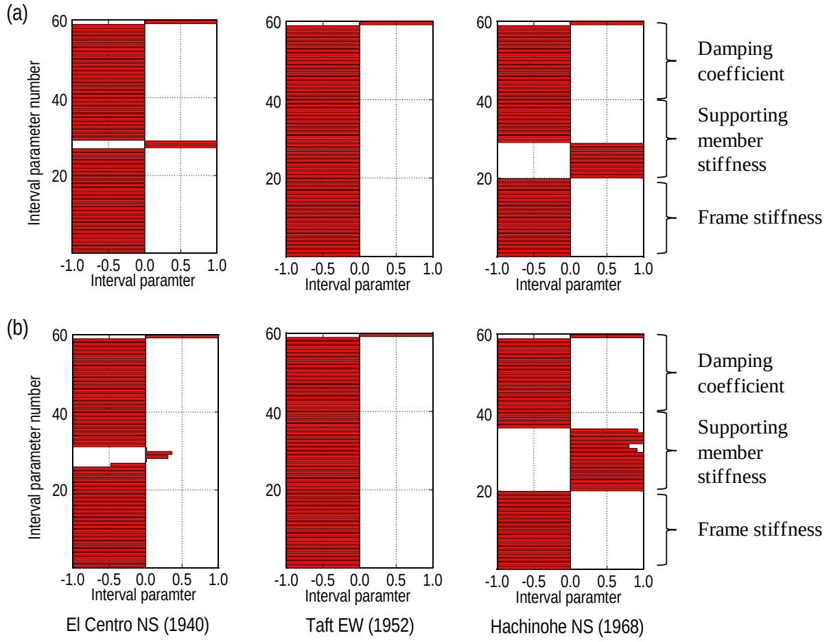
Fig.8 Comparison of critical interval parameters for upper bound of top horizontal displacement derived by first-order approximation with those of exact solution,
