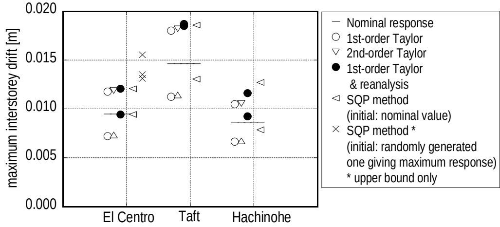
Fig.9 Comparison of evaluated bounds of maximum interstorey drift under uncertain structural parameters derived by Taylor series approximations with those derived by SQP method
