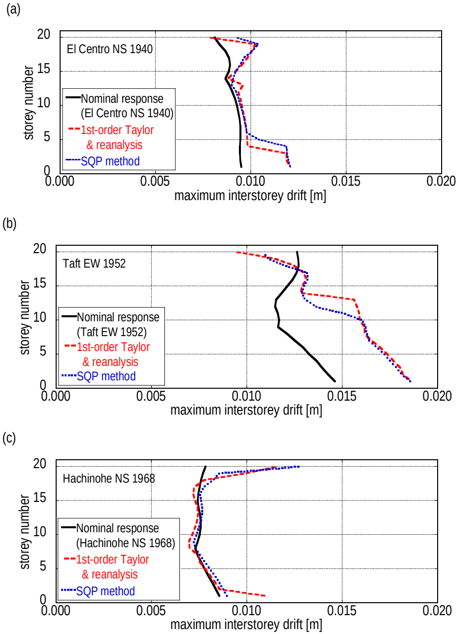
Fig.11 Comparison of maximum interstorey drifts under uncertain structural parameter sets derived by first-order Taylor approximation with those by SQP method, (a) El Centro NS 1940, (b) Taft EW 1952, (c) Hachinohe NS 1968
