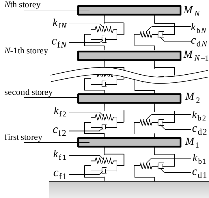
Fig.5 Structural model with passive dampers including supporting members
