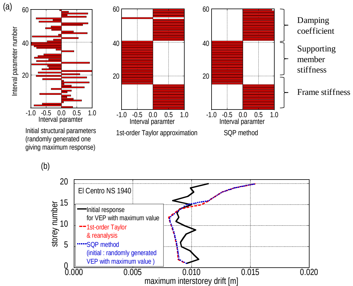
Fig.13 VEP method for maximum interstorey drift using initial structural parameter distribution derived by randomly generated one giving maximum response, (a) comparison of interval parameters, (b) comparison of maximum interstorey drift
