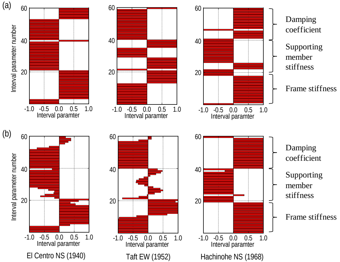
Fig.10 Comparison of critical interval parameters for upper bound of maximum interstorey drift derived by first-order approximation with those of exact solution
