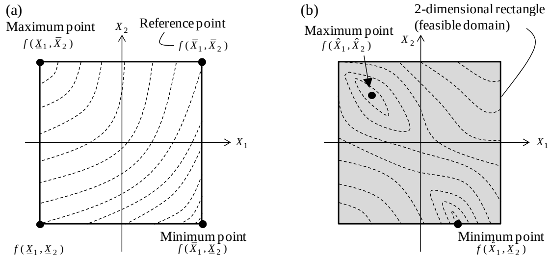
Fig.2 Relationship between the variation of objective function and the structural parameter combination, (a) example of ‘inclusion monotonic’, (b) example of ‘inclusion non-monotonic’
