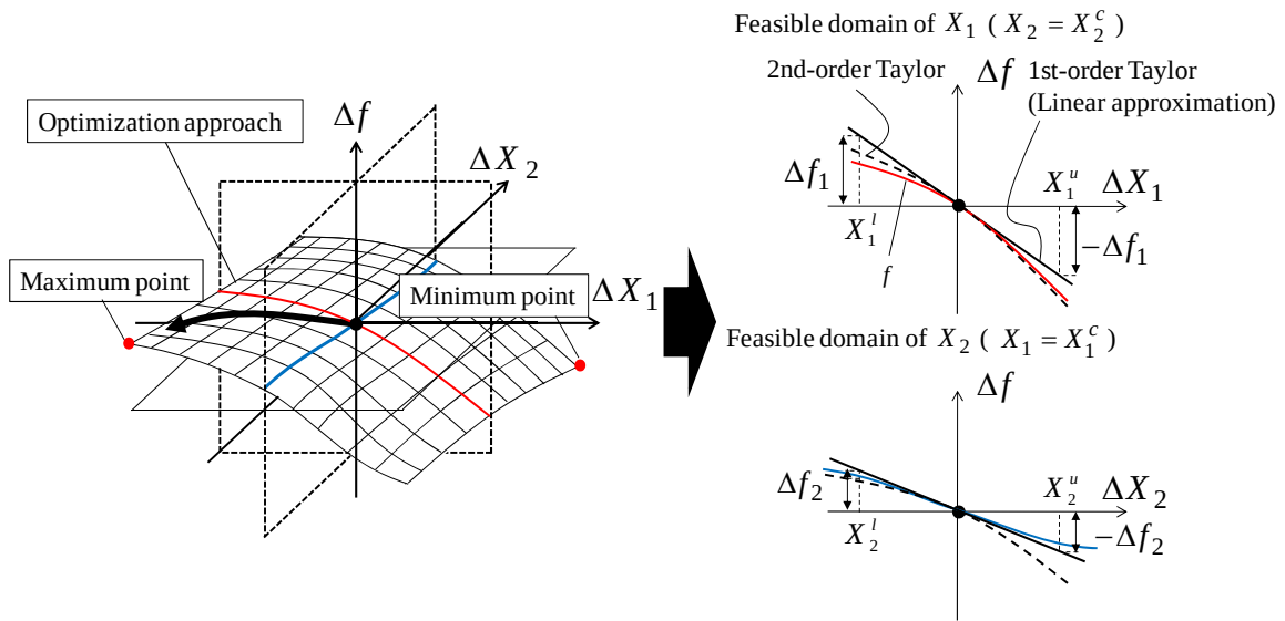
Fig.3 Concept of interval analysis method using Taylor series approximation
