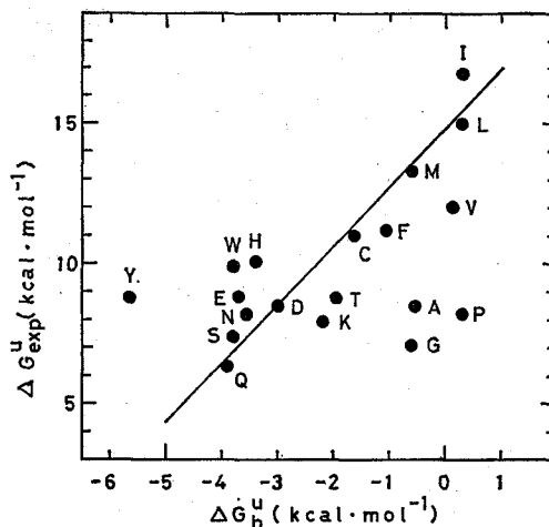
Fig. 7. Experimental unfolding free energy ( \Delta G_{exp}^u ) in water of 19 proteins ( T=25^\circ\text{C} at pH 7.0) substituted by each of 19 amino acids at position Glu 49 of tryptophan synthase \alpha subunit plotted against the hydration free energy of unfolding, \Delta G_h^u , of individual amino acid residues. The straight line represents least-square analyses of the values.
