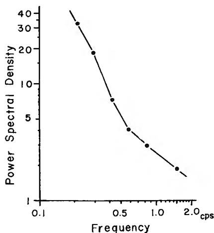
Fig. 3. Power spectrum of vorticity near the ground, (Shown in arbitrary unit).
