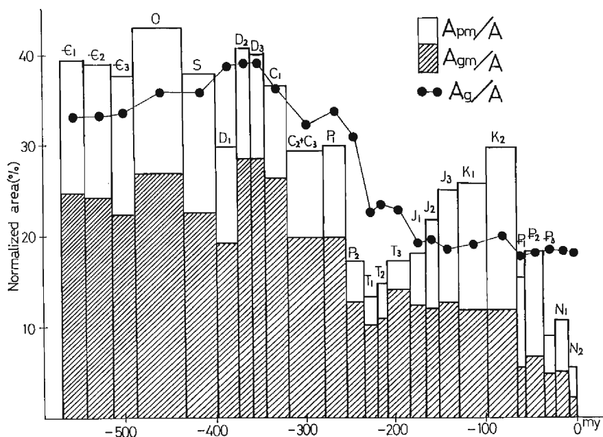
Fig. 2a World-wide temporal variation of the areas of geosynclinal regions ( A_g ) and marine basins covering platform regions ( A_{pm} ) and geosynclinal regions ( A_{gm} ), normalized to the total area of the present continents ( A ).
