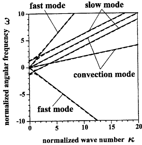
Fig 3. The dispersion relation in the limit of \alpha_0 \rightarrow 0 : u_{G0} = 0.5 , u_{L0} = 0.2 , \delta = 0.01 , \beta_1 = \beta_2 , and R_0 = 0.1\text{mm} . The dashed curves are those for \alpha_0 = 0.00001 .
