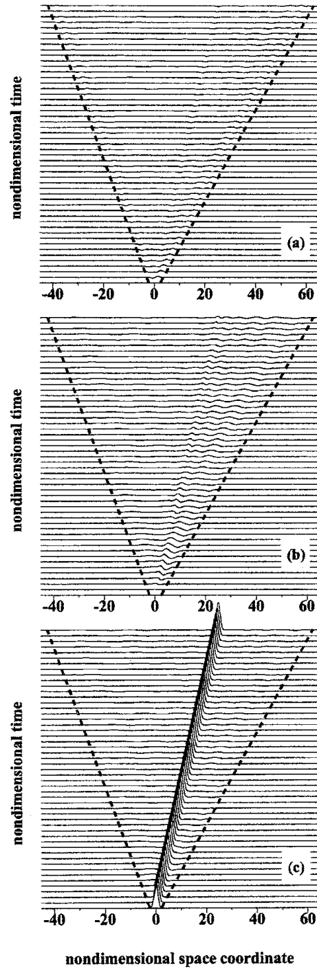
Fig 7. Wave profiles in the case of \alpha_0 = 0.00001 , u_{G0} = 0.5 , u_{L0} = 0.2 , \delta = 0.01 , \beta_1 = \beta_2 = \beta_3 = 0.5 , and R_0 = 0.1\text{mm} : (a) pressure, (b) bubble radius, (c) void fraction. The initial condition is \alpha = \exp(-x^2) and R = p_L = u_L = u_G = S = 0 at t = 0 .
