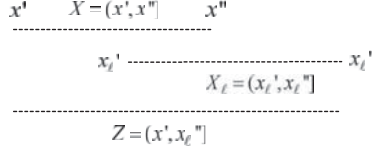
Figure 9: Two intervals X = (x', x''] and X_\ell = (x'_\ell, x''_\ell] in Proof of Lemma 5.1.
