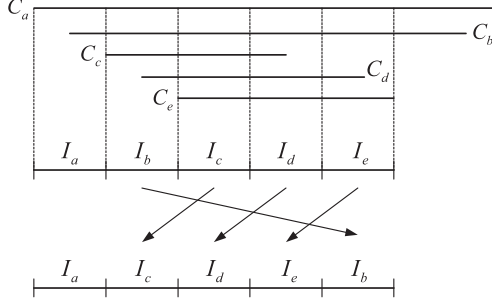
Figure 2: From a \mathcal{C} -unlocking permutation I_b, I_c, I_d, I_e in a maximal locked chain \mathcal{C} = I_a, I_b, I_c, I_d, I_e , we can obtain a chain \mathcal{C}' = I_a, I_c, I_d, I_e, I_b which is no longer locked. From another \mathcal{C} -unlocking permutation I_b, I_c, I_e , we can also obtain a chain \mathcal{C}'' = I_a, I_c, I_e, I_d, I_b which is no longer locked.
