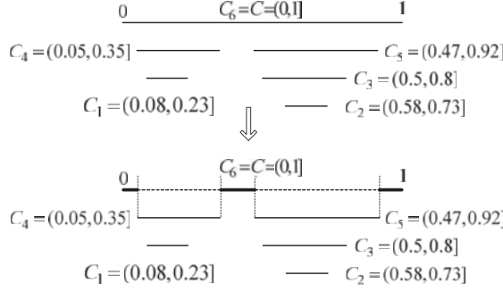
Figure 8: The cake-cutting problem can be reduced into two types of cake-cutting subproblems by cutting the cake C = (0, 1] at both endpoints of each maximal interval of minimum density: (i) one within each maximal interval of minimum density (players R_1 = \{1, 4\} and players R_2 = \{2, 3, 5\} ), and (ii) one with all valuations obtained by deleting all the valuation intervals contained in all maximal intervals of minimum density (players P = \{6\} ).
