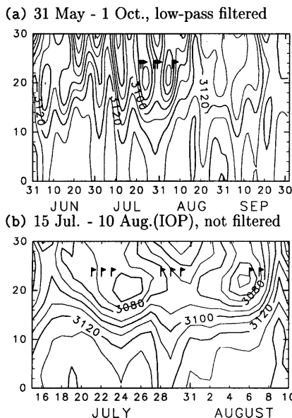
Fig. 3 Latitude-time cross sections of 700hPa geopotential height averaged between 85°E and 95°. (a) Low-pass filtered. From 31 May to 1 October. (b) Not filtered. Only for the IOP. Contour interval is 10m. Flags indicate the dates of 4 times daily observation.
