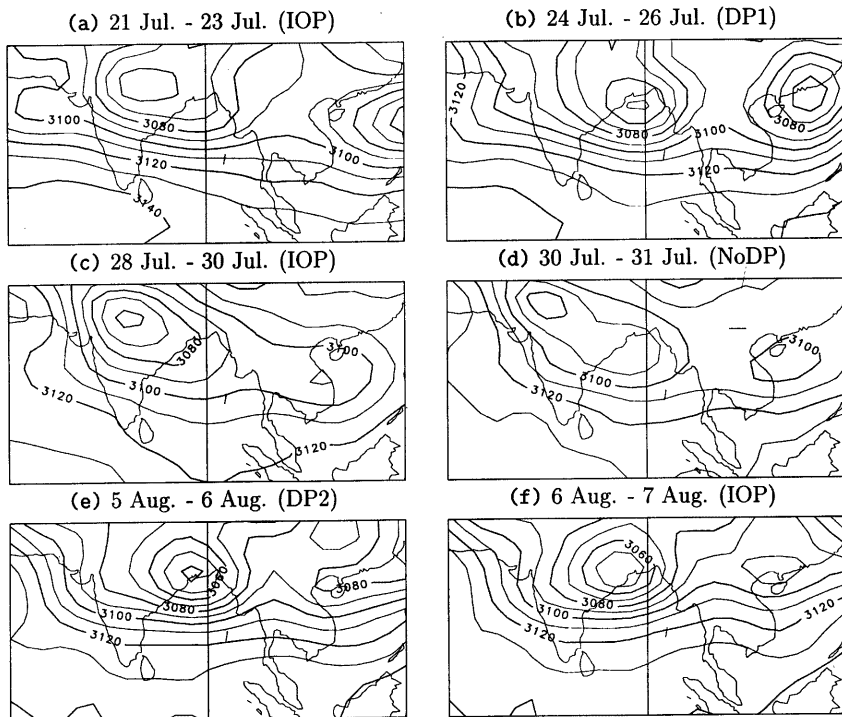
Fig. 4 Geopotential height to 700hPa over the South Asia for IOP periods ((a), (c), (f)), DP periods ((b), (e); when strong depressions are observed in Fig. 3), NoDP period ((d); when the geopotential heights are relatively high over the northern part of the Bay of Bengal in Fig. 3). Contour interval is 10m.
