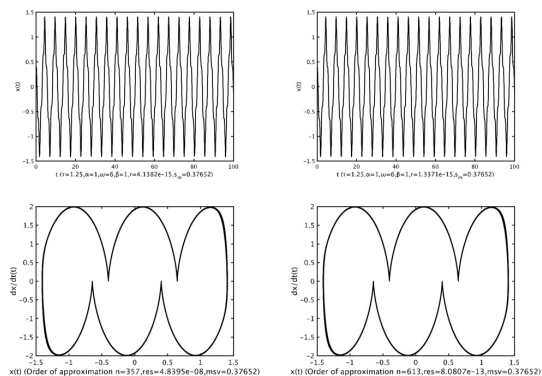
図 2. 1/5 Subharmonic ( \tau = 1.25, \alpha = 1, \kappa = 11, \beta = 1, \omega = 6 )
