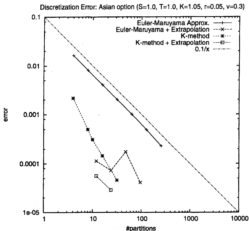
FIGURE 1. Approximation Error and number of partition. Asian option, BS-model
