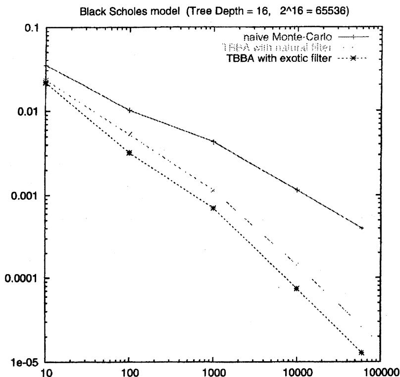
FIGURE 6. K-method with 3 sampling method: Convergence speed.
