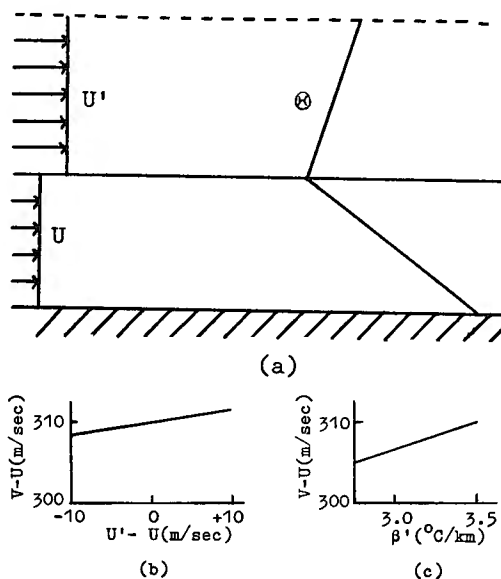
Fig. 3 Two-layer model (a). (b): the wave solution for \beta=6.8^{\circ}\text{C}/\text{km} , \theta_0=26^{\circ}\text{C} and \beta'=3.4^{\circ}\text{C}/\text{km} . (c) the solution for \beta=6.8^{\circ}\text{C}/\text{km} , \theta_0=26^{\circ}\text{C} and U=U' .
