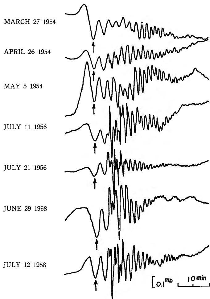
Fig. 1 Microbarograms due to the nuclear explosions.
