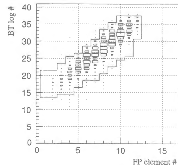
Figure 2.21: Correlation between the FP element number and the BT log number for K^+ 's of p_{K^+} > 1.1 \text{ GeV}/c . The region surrounded by a solid line was selected by the matrix coincidence logic.
