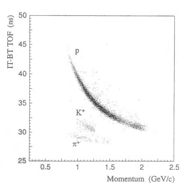
Figure 3.7: Plot of momentum versus TOF for the outgoing particles. Three loci correspond to \pi^+ , K^+ , and protons, respectively, as indicated.
