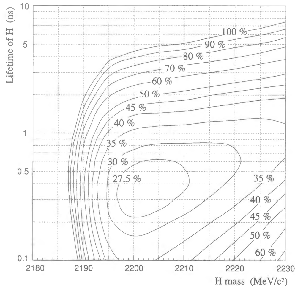
Figure 3.55: Contour plot of 90% C.L. upper limits on the product of the branching ratios, R (= Br[(\Xi^-, {}^{12}\text{C})_{\text{atom}} \rightarrow HX] \cdot Br[H \rightarrow \Lambda n]) , where X was assumed to be {}^{11}\text{B}(\text{g.s.}) .
