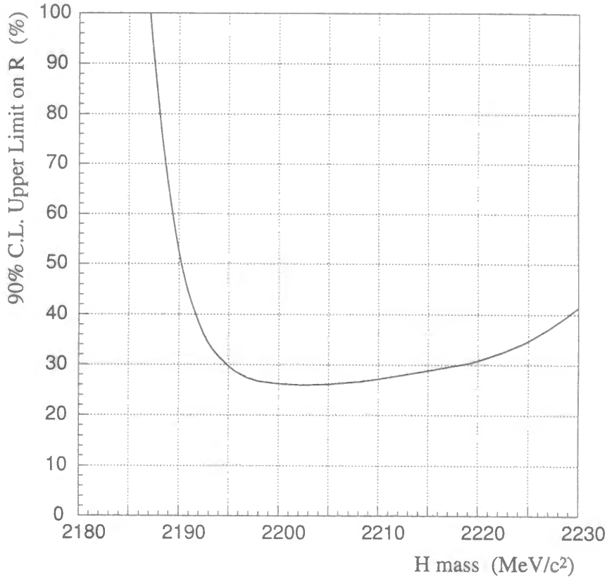
Figure 3.54: 90% C.L. upper limits on the product of the branching ratios, R (= Br[(\Xi^-, {}^{12}\text{C})_{\text{atom}} \rightarrow HX] \cdot Br[H \rightarrow \Lambda n]) , as a function of the H mass in the case of the H lifetime of 0.4 ns. The residual of the H formation ( X ) was assumed to be {}^{11}\text{B}(\text{g.s.}) .
