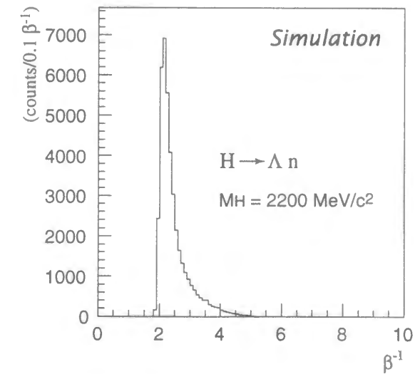
Figure 3.46: Simulated \beta^{-1} spectrum in H \rightarrow \Lambda n decay with an assumed H mass of 2200 MeV/ c^2 .
