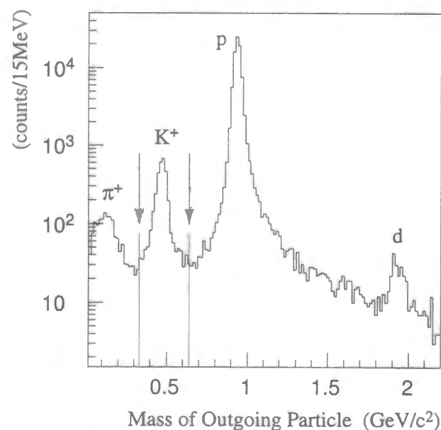
Figure 3.9: Mass spectrum of the outgoing particles. The events between the arrows were extracted as the K^+ sample in the data reduction.
