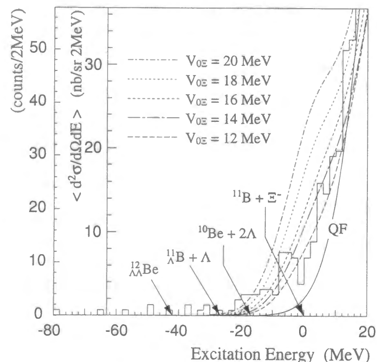
Figure 3.28: Excitation-energy spectrum of ^{11}\text{B} + \Xi^- around the threshold with several curves of the theoretical calculations for \Xi^- hypernuclear production assuming Woods-Saxon potential. The curves in case of the Woods-Saxon potential well depth V_{0\Xi} = 12, 14, 16, 18 , and 20 \text{ MeV} are presented. The simulation result which contains the contribution of only quasi-free \Xi^- production is shown with the label “QF”. The energy thresholds of ^{10}\text{Be} + 2\Lambda and ^{11}\text{B} + \Lambda and the expected location of the ground state of ^{12}_{\Lambda\Lambda}\text{Be} are also indicated with arrows.
