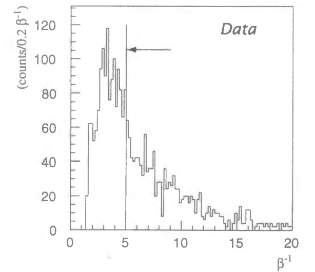
Figure 3.47: Experimental \beta^{-1} distribution of the current analysis sample. The solid line shows the cut position.
