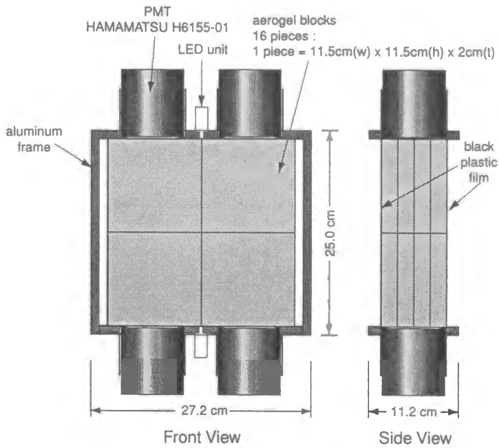
Figure 2.7: Schematic drawing of FC.
