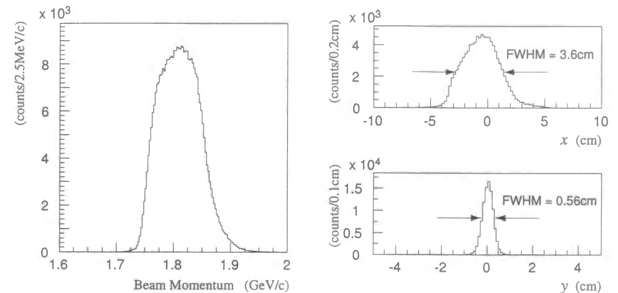
Figure 3.1: Momentum distribution of the beam particles.
