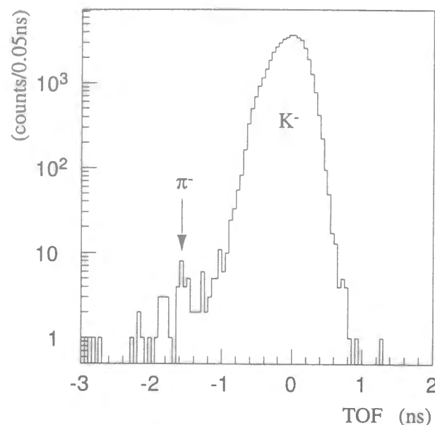
Figure 3.3: Spectrum of the TOF between MT and IT for particles passed through the online K^- selection by the aerogel Čerenkov counter IC.
