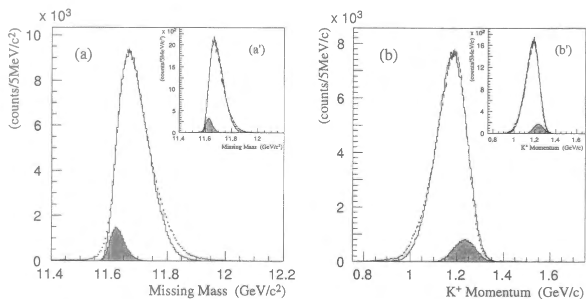
Figure 3.22: Comparison between the Monte Carlo simulation and the experimental data in terms of (a): the missing mass for ^{12}\text{C}(K^-, K^+) kinematics and (b): the K^+ momentum. The solid lines show the simulation results and the error bars show the experimental data. Relatively loose cuts were applied to produce the data histograms of (a) and (b), while quite tight cuts were applied for (a') and (b') (see the text).
