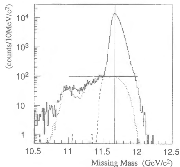
Figure 3.39: Missing mass spectrum of the (K^-, K^+) event sample. The solid line shows the one which passed the primary loose cuts described in Section 3.13.1, while the dashed line represents the one in which the further cut on K^+ momentum was applied. The dotted line shows the missing mass spectrum of protons with ^{12}\text{C}(K^-, K^+) kinematics scaled to fit the solid line (see the text).
