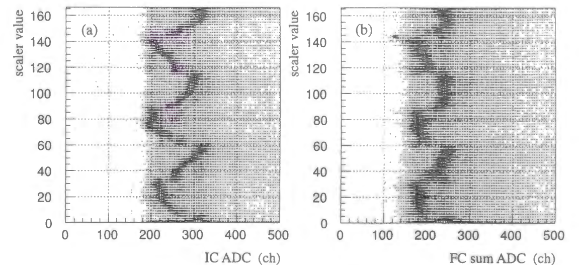
Figure C.1: ADC pedestal fluctuation depending on 60Hz phase of the AC noise for the aerogel Čerenkov counters IC(a) and FC(b). Signals from FC were analog-summed over its four PMT channels. The scaler value corresponds to time interval from the reset time with a unit of 0.1 ms.
