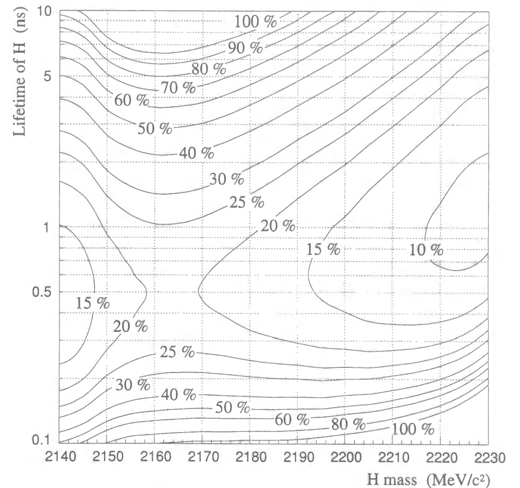
Figure 3.42: Contour plot of 90% C.L. upper limits on the product of the branching ratios, R (= Br[(\Xi^-, {}^{12}\text{C})_{\text{atom}} \rightarrow HX] \cdot Br[H \rightarrow \Sigma^- p]) , where X was assumed to be {}^{11}\text{B}(\text{g.s.}) .
