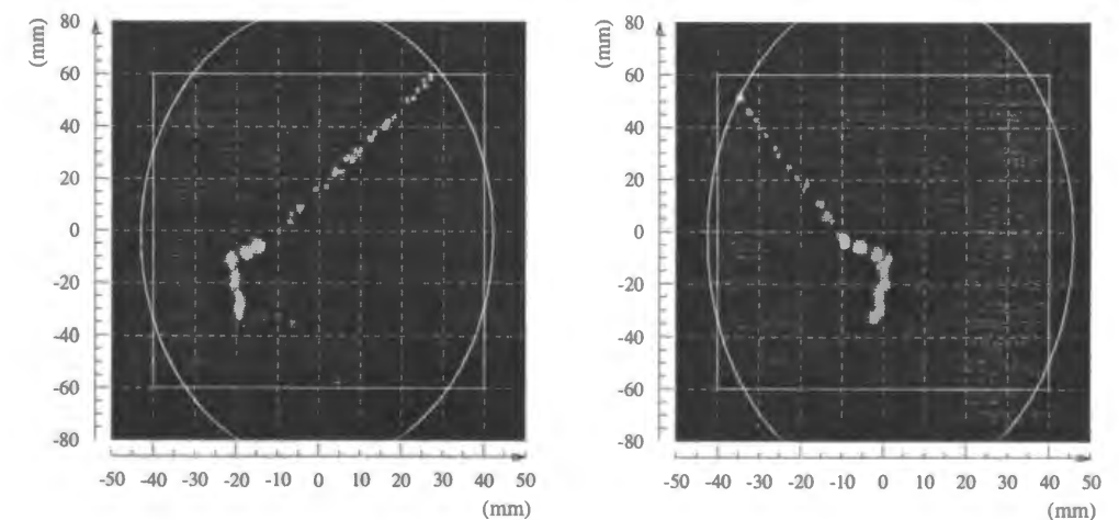
Figure 3.36: Example of the simulated image data for the sequential decay H \rightarrow \Sigma^- p , \Sigma^- \rightarrow n\pi^- . Two images correspond to the left and right views of the SCIFI block respectively.
