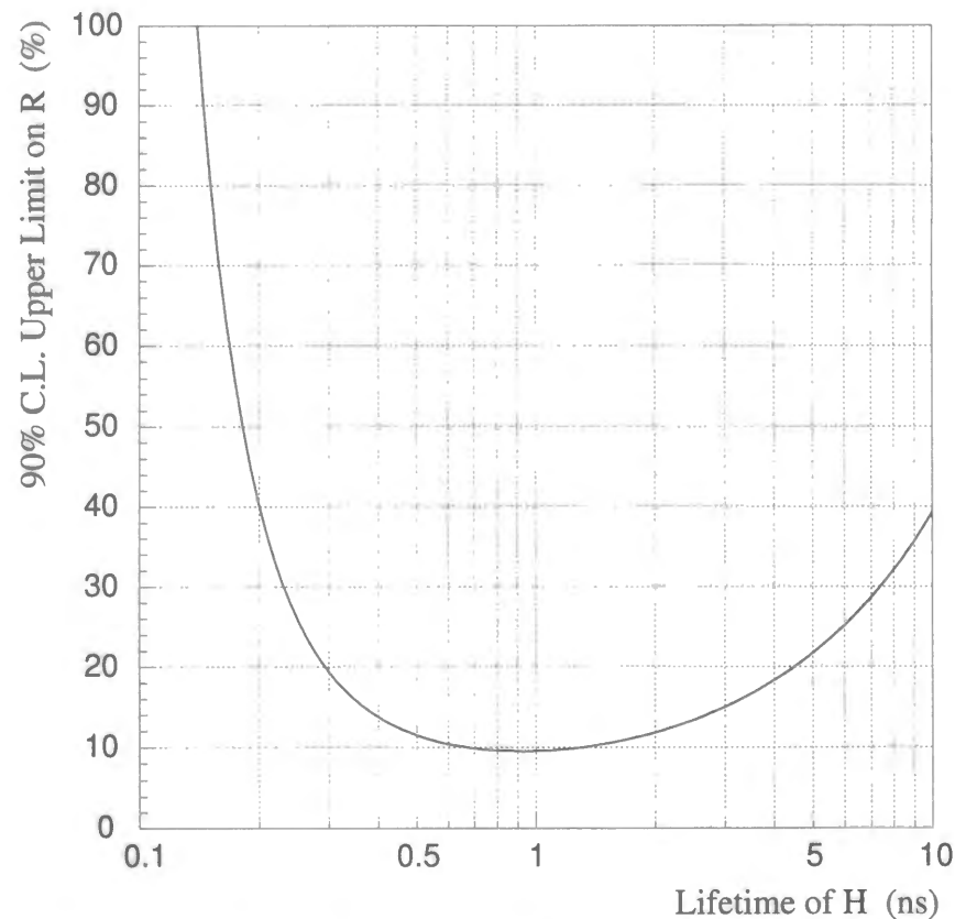
Figure 3.41: 90% C.L. upper limits on the product of the branching ratios, R (= Br[(\Xi^-, {}^{12}\text{C})_{\text{atom}} \rightarrow HX] \cdot Br[H \rightarrow \Sigma^- p]) , as a function of the H lifetime in the case of the H mass of 2220 \text{ MeV}/c^2 . The residual of the H formation ( X ) was assumed to be {}^{11}\text{B}(\text{g.s.}) .
