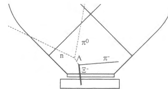
Figure 3.51: Example of background events included in the ' \Lambda decay' events. When a \Xi^- comes into and decays in the SCIFI block, then the resultant \Lambda decays into neutrals or decays out of the SCIFI block, the event has the same topology as that of the \Lambda decay.
