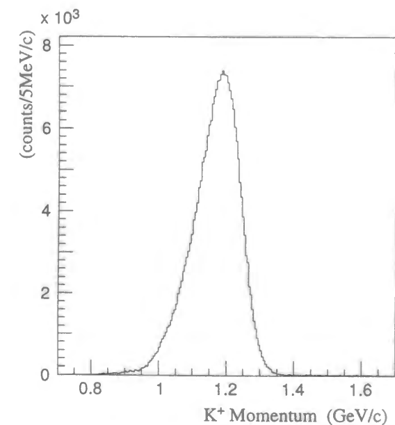
Figure 3.8: Momentum spectrum of the outgoing K^+ . The low momentum region is out of the acceptance of the spectrometer (see the text).
