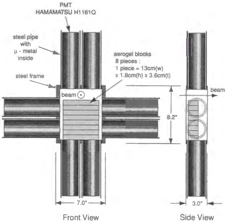
Figure 2.8: Schematic drawing of FC0.
