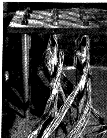
Photo. 1 Piles and strain gauges.
