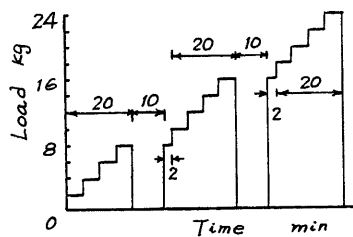
Fig. 4 Lateral loading cycles.
