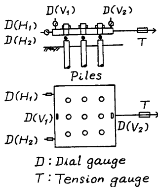
Fig. 5 Piles and gauges.
