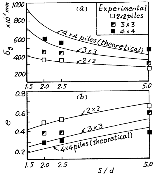
Fig. 10 Test results and theoretical curves for Box arrangement piles: (a) pile deflections at the loaded end; (b) group efficiencies.
