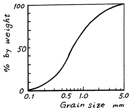
Fig. 2 Grain size distribution curve.
