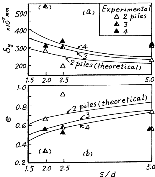
Fig. 9 Test results and theoretical curves for Series arrangement piles:
