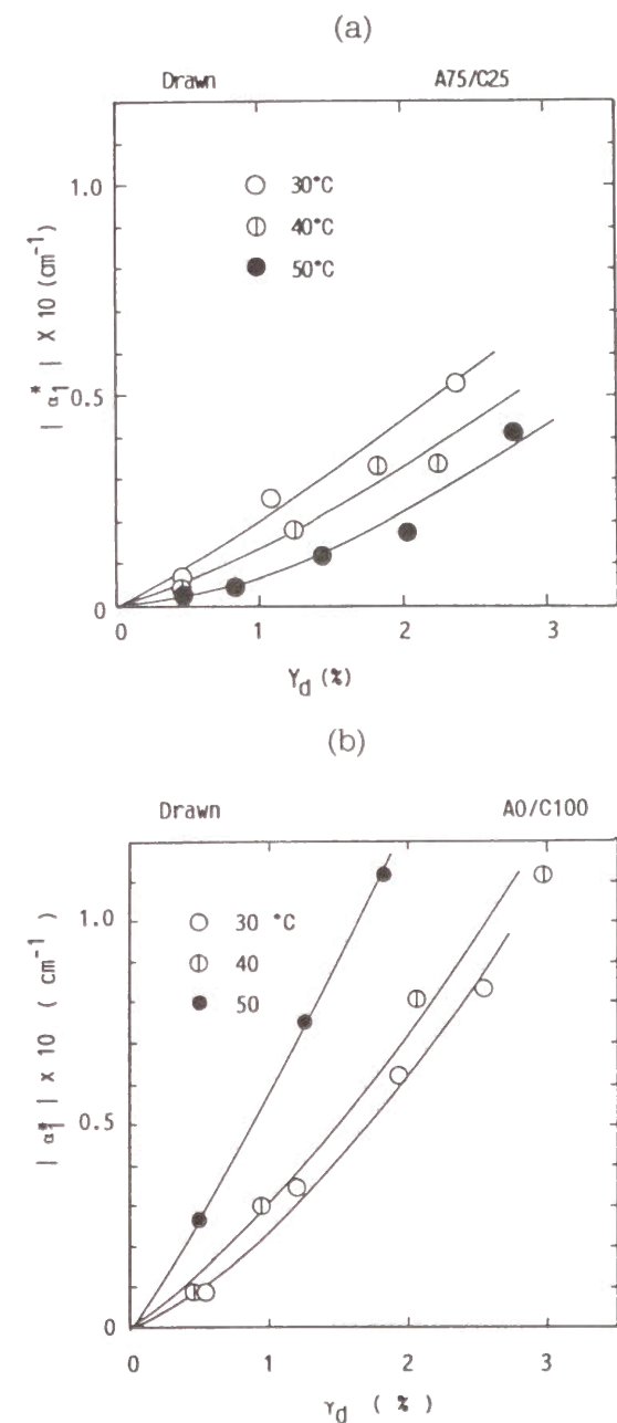
Fig.5-8 Variation of |a^*| with dynamic strain amplitude \gamma_d for drawn A75/C25 and A0/C100 films.
