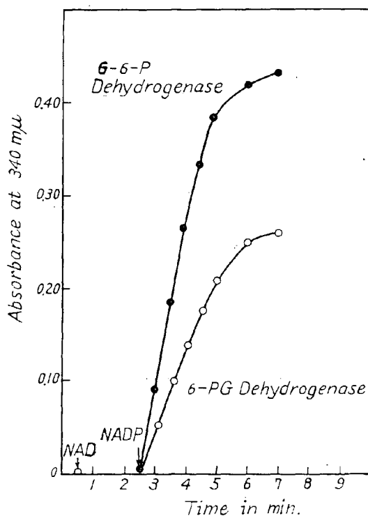
Fig. 2. Specificity of enzyme Enzyme concentration; 3.0 mg protein/ ml. NAD or NADP was added at the points shown. ( Phyllostachys pubescens )
