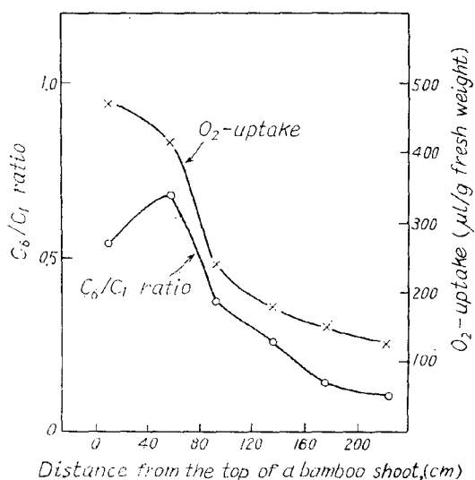
Fig. 4. Pattern of respiratory breakdown of glucose-1- 14 C and -6- 14 C. ( Phyllostachys pubescens )
