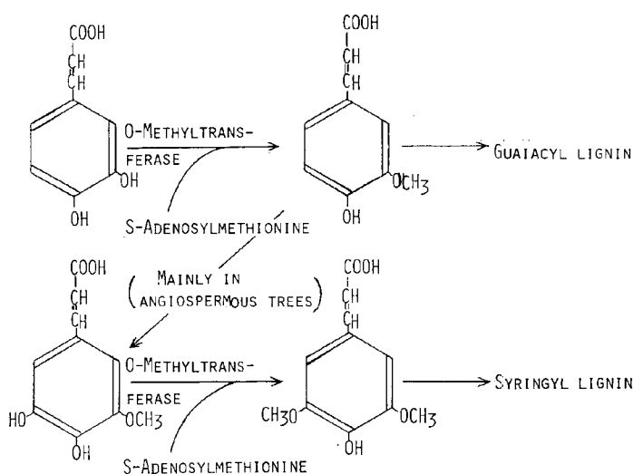
Fig. 13. Metabolic differences in formation of guaiacyl- and syringyl lignins in gymnospermous- and angiospermous trees.
