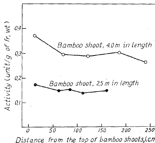
Fig. 5. Activity of 5-Dehydroquinase hydro- lyase in different parts of bamboo. ( Phyllostachys pubescens )
