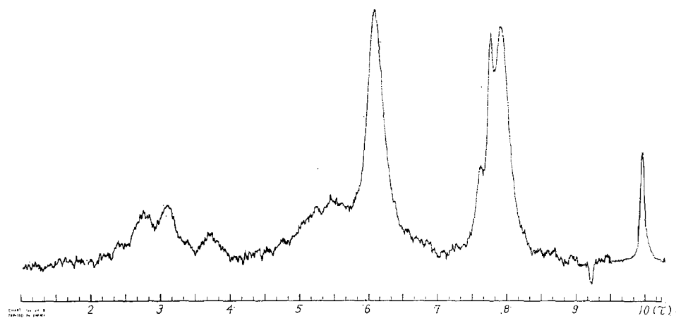
Fig. 16. NMR spectrum of the acetylated MWL of a poplar ( Populus nigra ).
