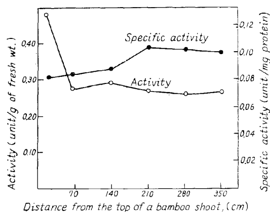
Fig. 7. Activity changes in 5-dehydroshikimate reductase in different parts of bamboo. ( Phyllostachys pubescens )
