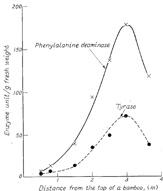
Fig. 10. Activity changes in phenylalanine deaminase and tyrase of different portions of a bamboo. ( Phyllostachys pubescens )
