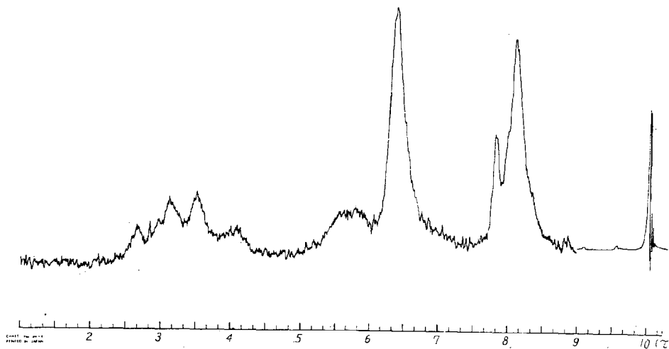
Fig. 17. NMR spectrum of the acetylated MWL of a bamboo ( Phyllostachys pubescens ).
