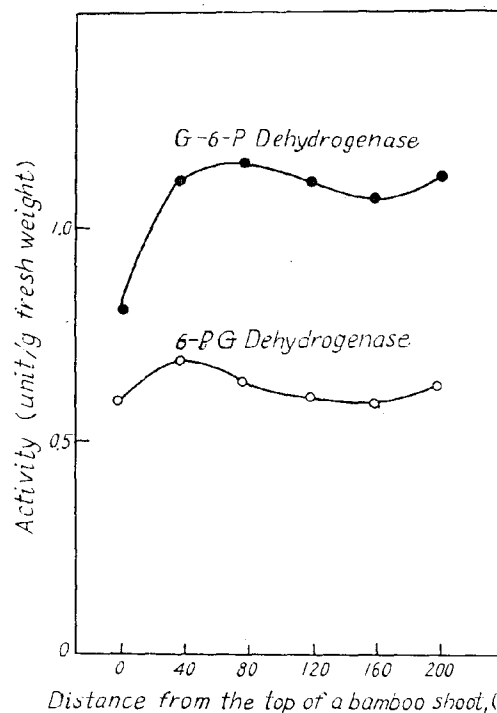
Fig. 3. Changes in activity of G-6-P and 6-PG dehydrogenases in different parts of bamboo. ( Phyllostachys pubescens )
