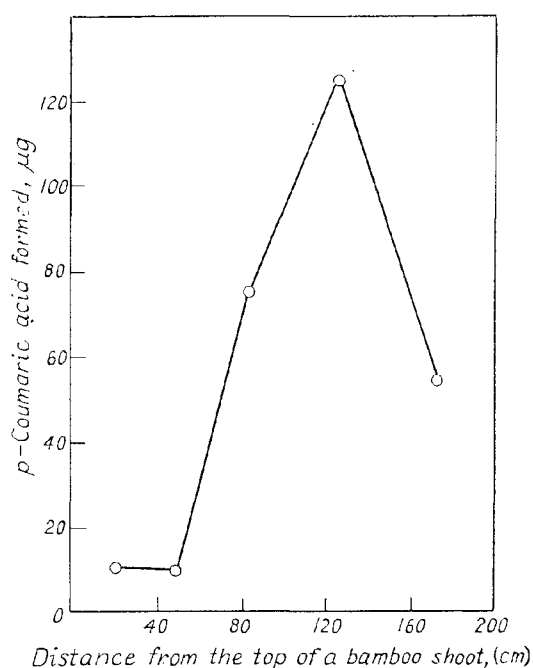
Fig. 11. Pattern of cinnamic acid hydroxylating activity in different tissue samples. ( Phyllostachys pubescens )
