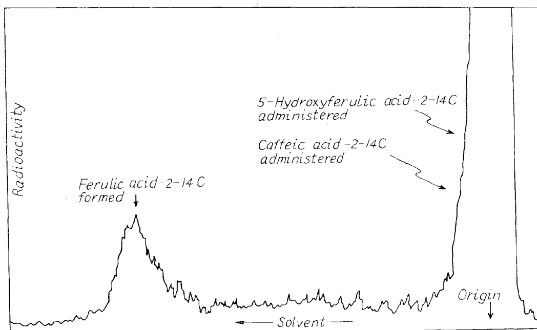
Fig. 12. Selective methylation for dihydroxycinnamic acid by Ginkgo biloba . Solvent, toluene, acetic acid and water (4:1:5, v/v, organic layer).
