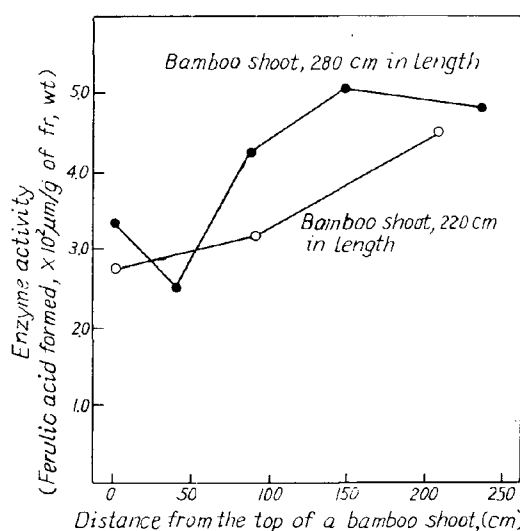
Fig. 14. Changes in activity of O-methyltransferase. ( Phyllostachys reticulata )
