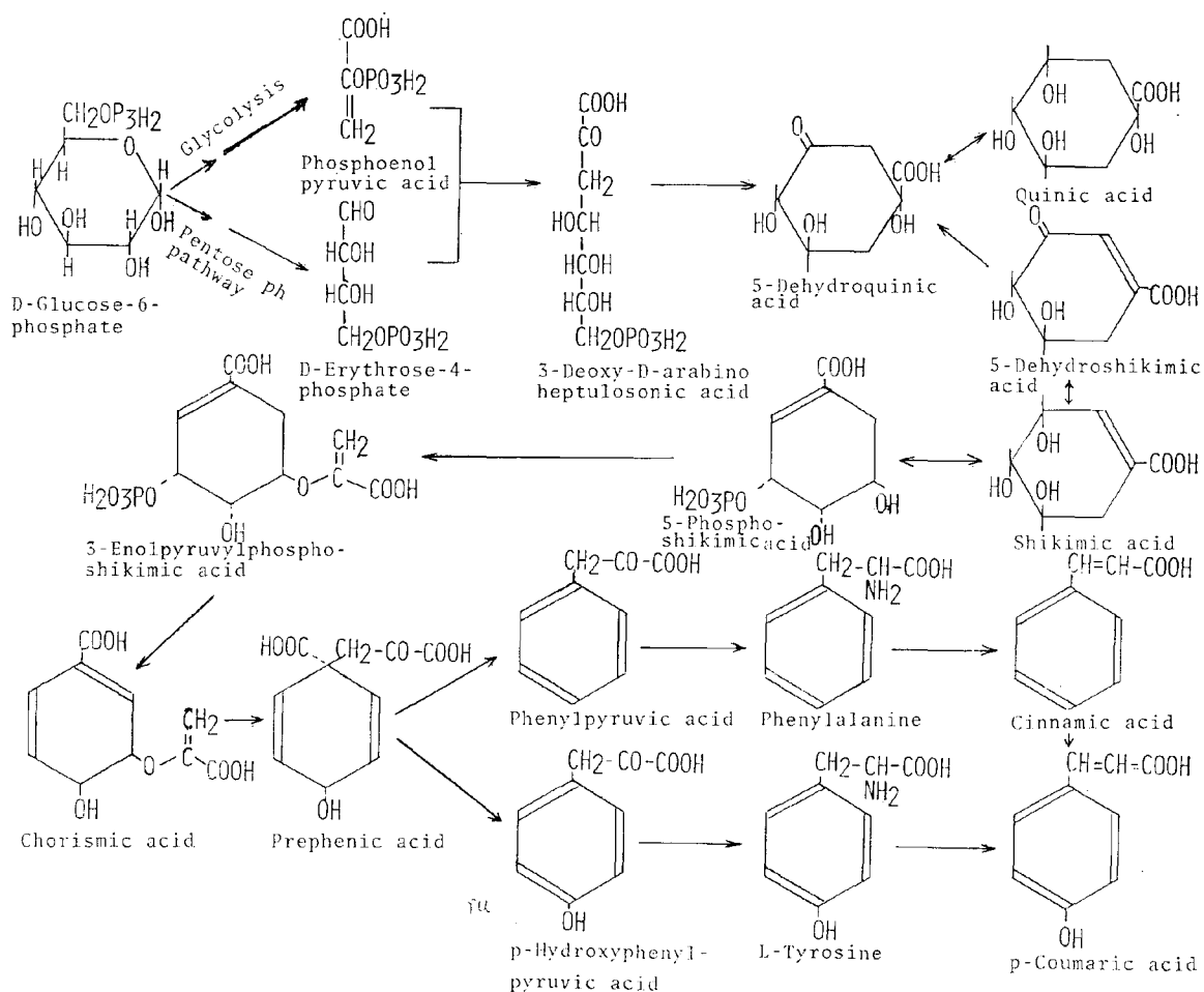
Fig. 1. Biosynthesis of the phenylpropanoid amino acids and cinnamic acids from glucose-6-phosphate.
