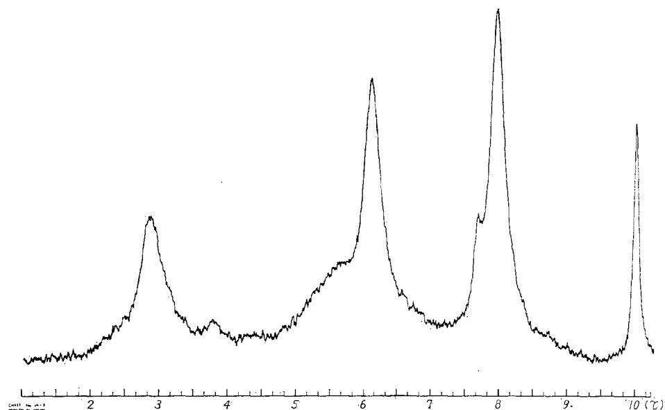
Fig. 15. NMR spectrum of the acetylated MWL of Japanese red pine ( Pinus densiflora ).
