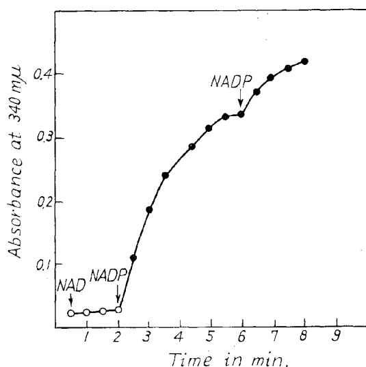
Fig. 6. Specificity of 5-DHS reductase Enzyme concentration; 13.2mg protein/ ml. NAD or NADP was added at the points shown. ( Phyllostachys pubescens )
