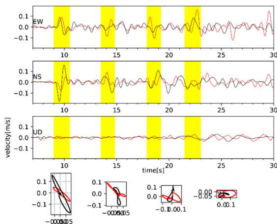
Fig. 5 Comparison of observed (black) and simulated (red) velocity waveforms and particle motion at station OSKP45.
