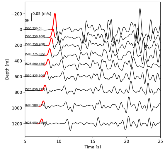
Fig. 3 Simulated waveforms of the first reflected wave packet arriving at OSKP45, along the subsequent downward path retraced in reverse from the surface to the basement.
