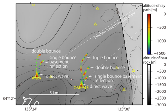
Fig. 4 Figure 4. Ground-surface projection of the propagation paths of the direct and reflected wave packets arriving at stations AMA and OSKP45 in the simulated wavefield.
