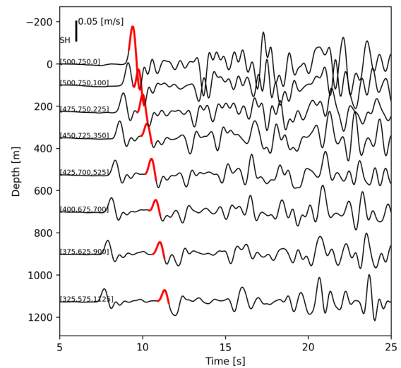
Fig. 2 Simulated waveforms of the first reflected wave packet arriving at OSKP45, along the upward path retraced in reverse from the basement back to the surface.
