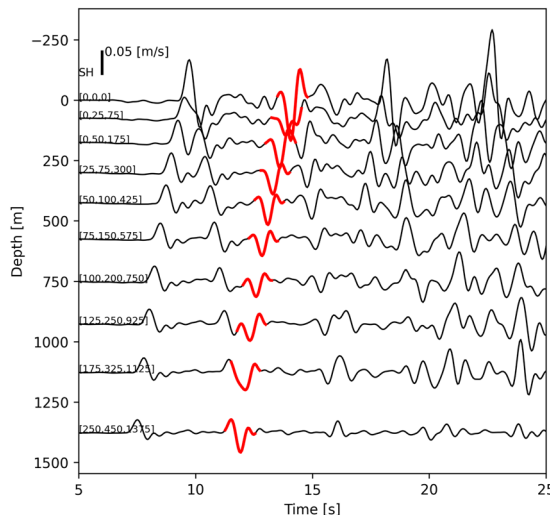
Fig. 1 Simulated waveforms of the first reflected wave packet arriving at OSKP45, along the downward path retraced in reverse from the surface to the basement. Traces are shifted by depth, and red traces indicate the target wave packet used for semblance analysis.
