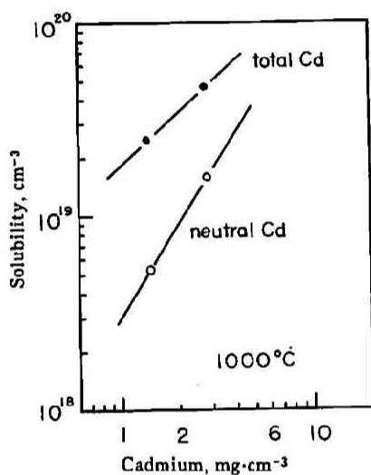
Fig. 4 Solubility of Cd vs amounts of added Cd at 1,000°C
