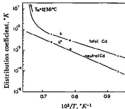
Fig. 3 Distribution coefficient of Cd in GaAs ●: Data points of total Cd calculated from the experimental solubilities and theoretical liquidus line ○: Neutral Cd calculated from the solubilities of neutral Cd and liquidus line
