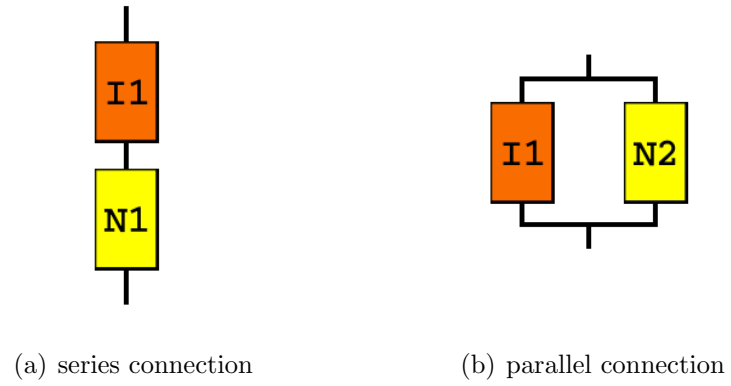
Figure 1: Basic series and parallel connections of multicell battery with two different cells.
