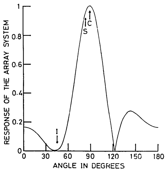
Fig.II.6.16 Radiation pattern of the adaptive array after 1000 iterations. (see Table II.6.3)
