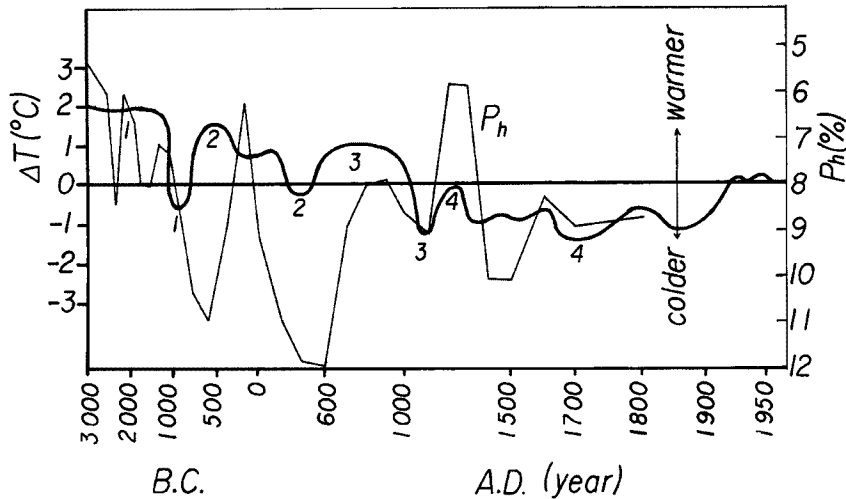
Fig. 2. Temperature change during the last 5000 years in China, expressed as deviation from the present day mean by Chu 10 and averaged climate change index P_h 16 (the numbers show the four alternating warm and cold periods).
