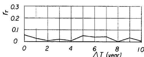
Fig. 12. Serial correlation coefficient of occurrence of flooding in Japan and in China.
