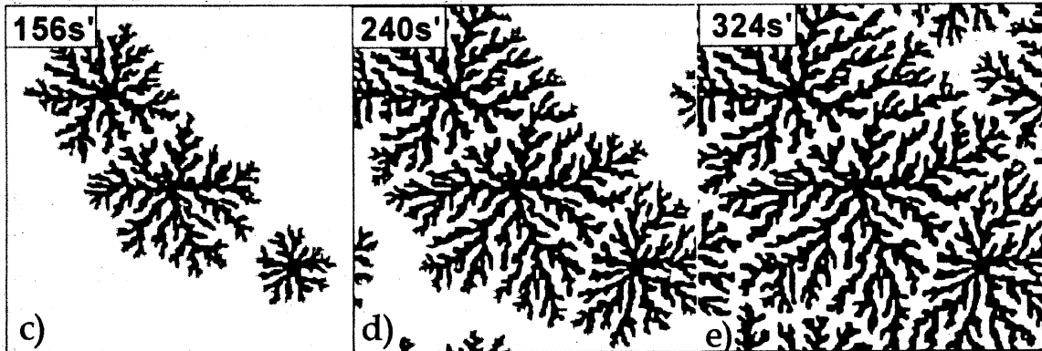
Fig. 4. Pattern evolution of c-Si aggregates in Al (50nm)/Si (25nm)/SiO 2 bilayer films: SEM images after annealing at 498 K for 28.8 ks (a) and 460.8 ks (b); simulation results based on the phase-field method (c, d, e).
