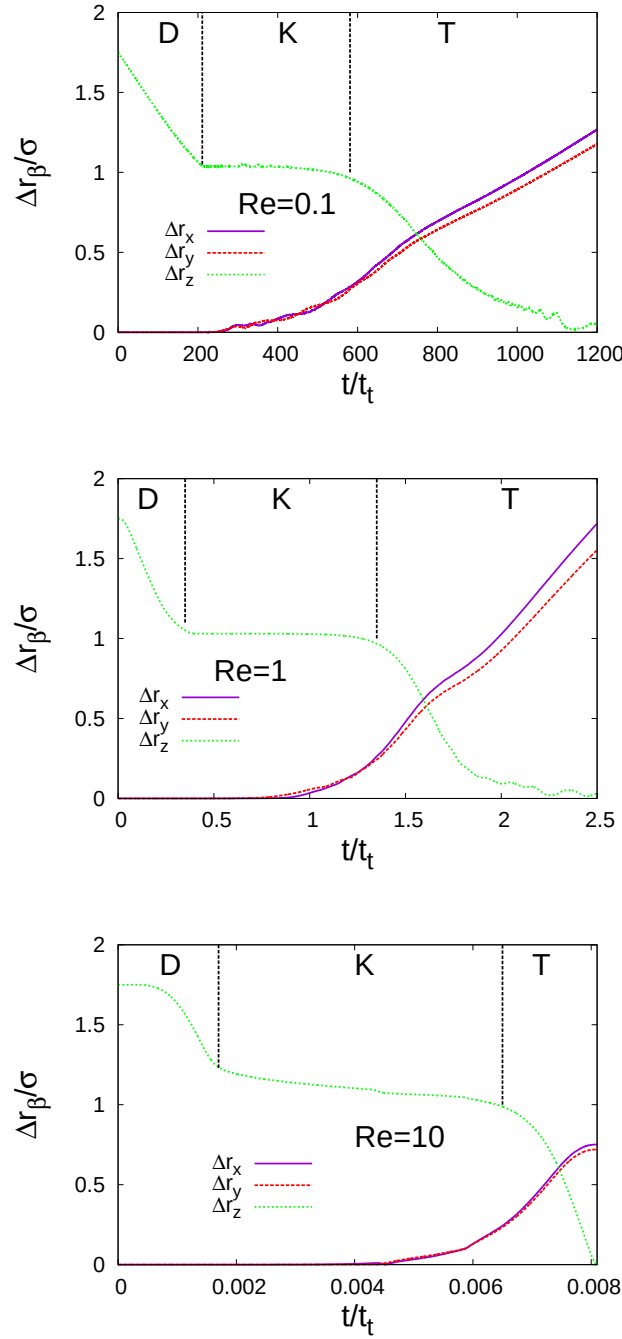
FIGURE 4.2: Distance between two particles in all three directions \Delta r_\beta , where \beta \in x, y, z , as a function of terminal time for three different Re. These three figures are divided into three sections, where “D” shows the drafting, “K” shows the kissing and “T” shows the tumbling phase of the DKT mechanism.
