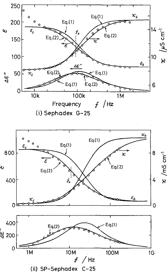
Fig. 2. Frequency dependence of relative permittivity \epsilon , electrical conductivity \kappa , and loss factor \Delta\epsilon'' = (\kappa - \kappa_i)/(2\pi f\epsilon_0) for beds of (i) Sephadex G-25 beads in a sodium form dispersed in water at 22.4°C and (ii) SP-Sephadex C-25 beads in a sodium form dispersed in water at 24.0°C.
