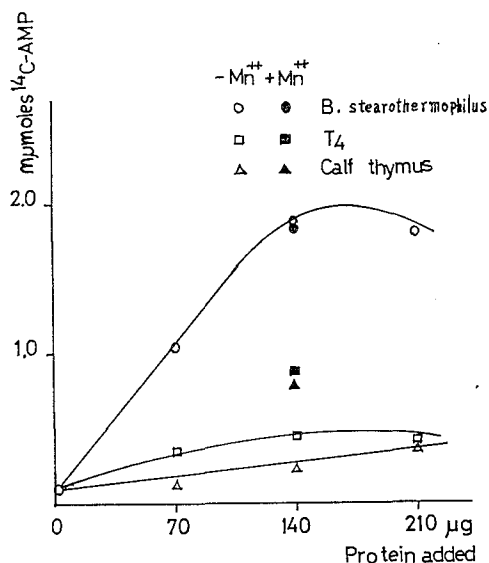
Fig. 5. The template activity of DNAs from different sources.
