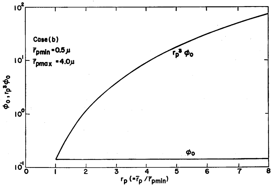
Fig. 2. Functions \phi_0(r_p) and r_p^3 \phi_0(r_p) for Case (b).
