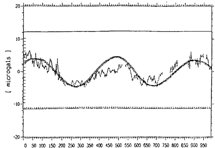
Fig.8 Gravity residuals after removal of the quadratic trend and the large irregular changes from original data(solid line) and theoretically estimated gravity changes at Kyoto induced by the polar motion(circles)
